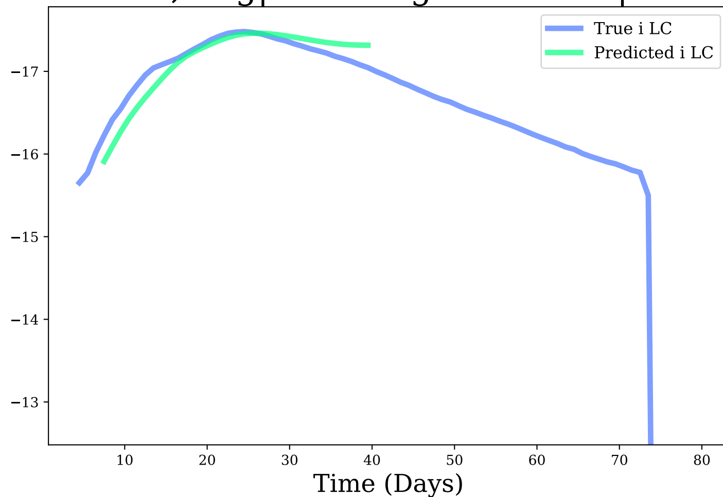
i-band, Avg|Max Mag Diff: 0.13 | 0.32
