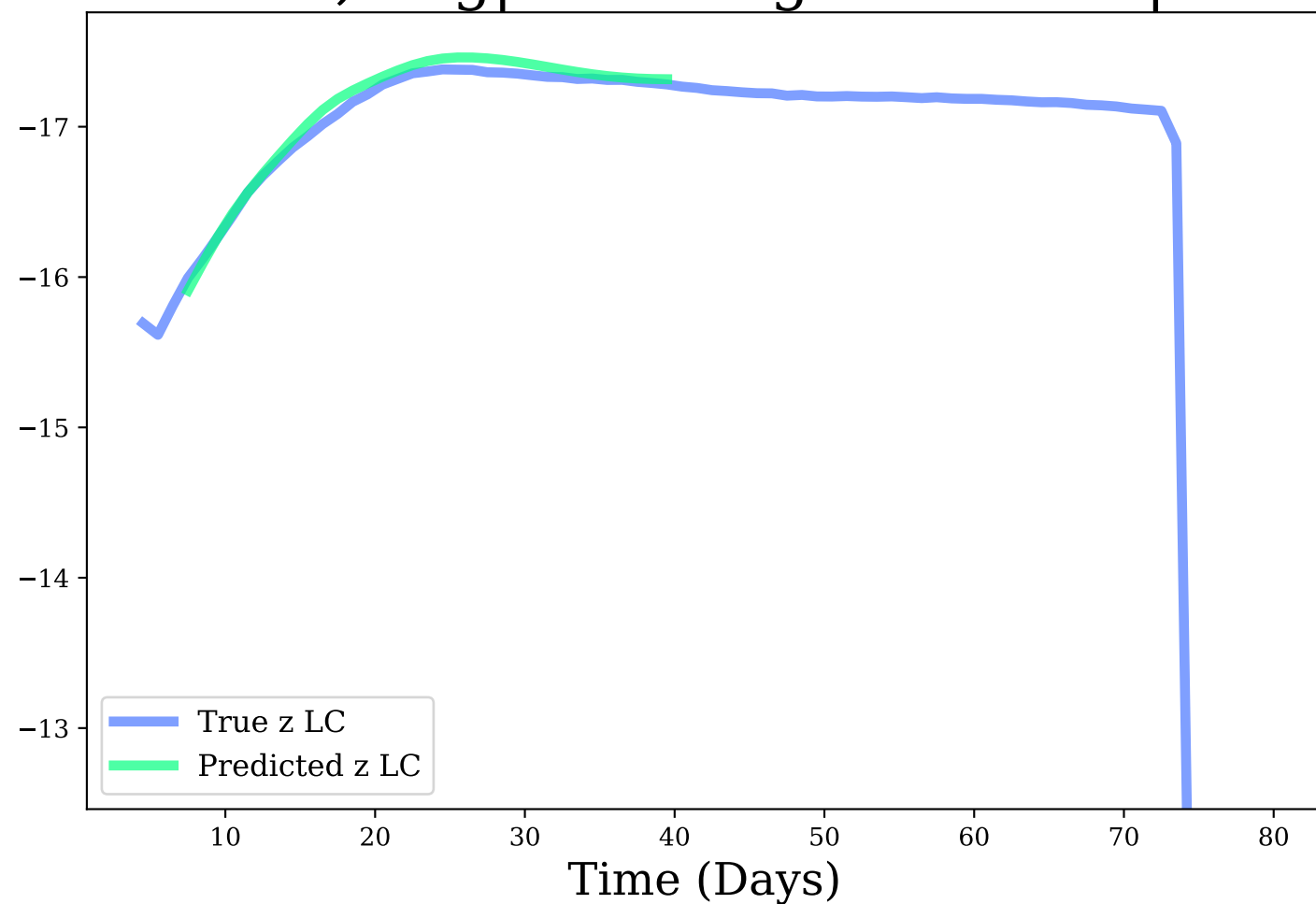
z-band, Avg|Max Mag Diff: 0.05 | 0.1
