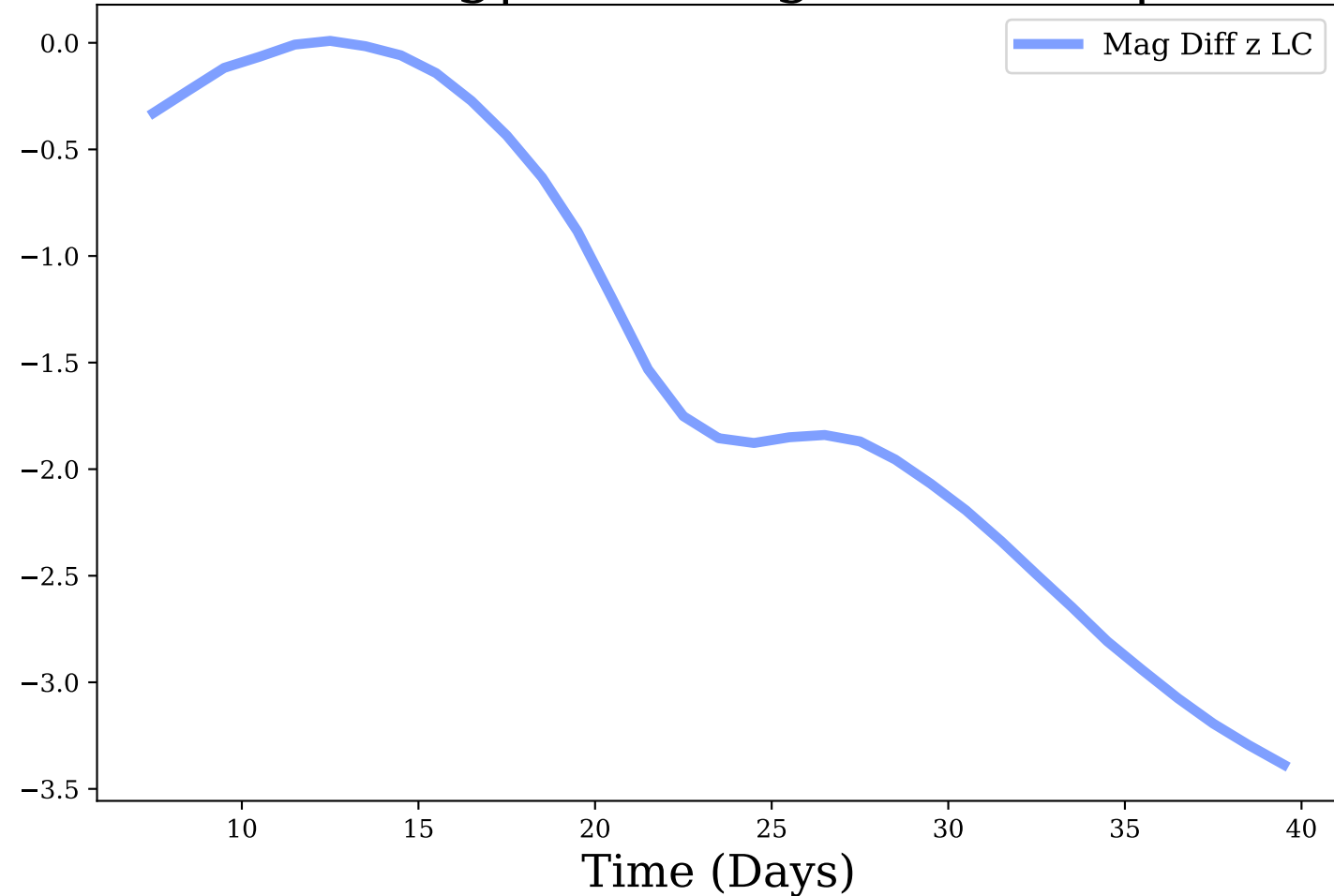
z-band, Avg|Max Mag Diff: -1.5 | 3.39
