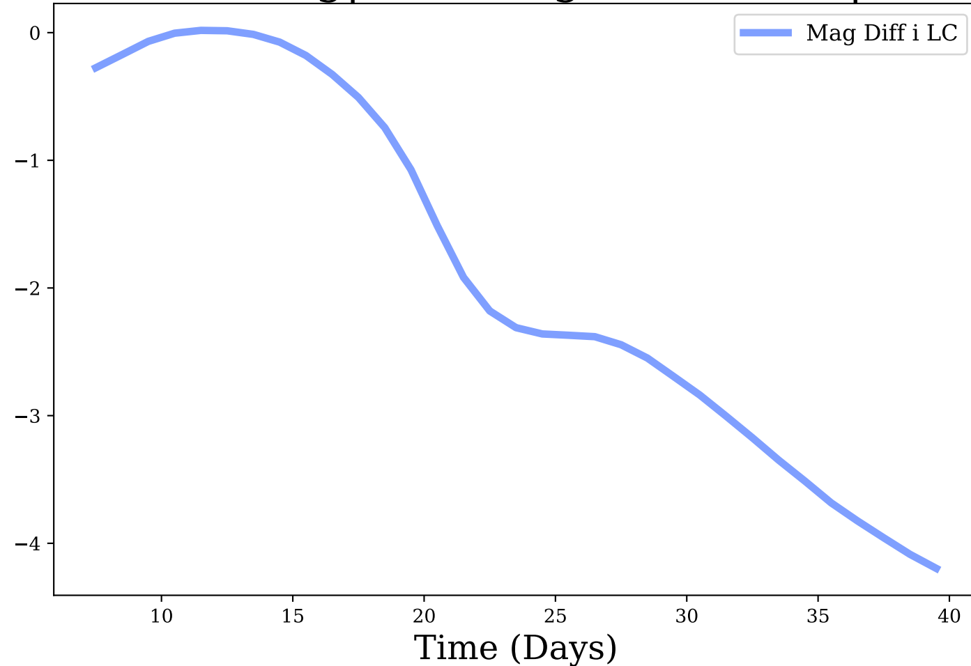
i-band, Avg|Max Mag Diff: -1.87 | 4.2
