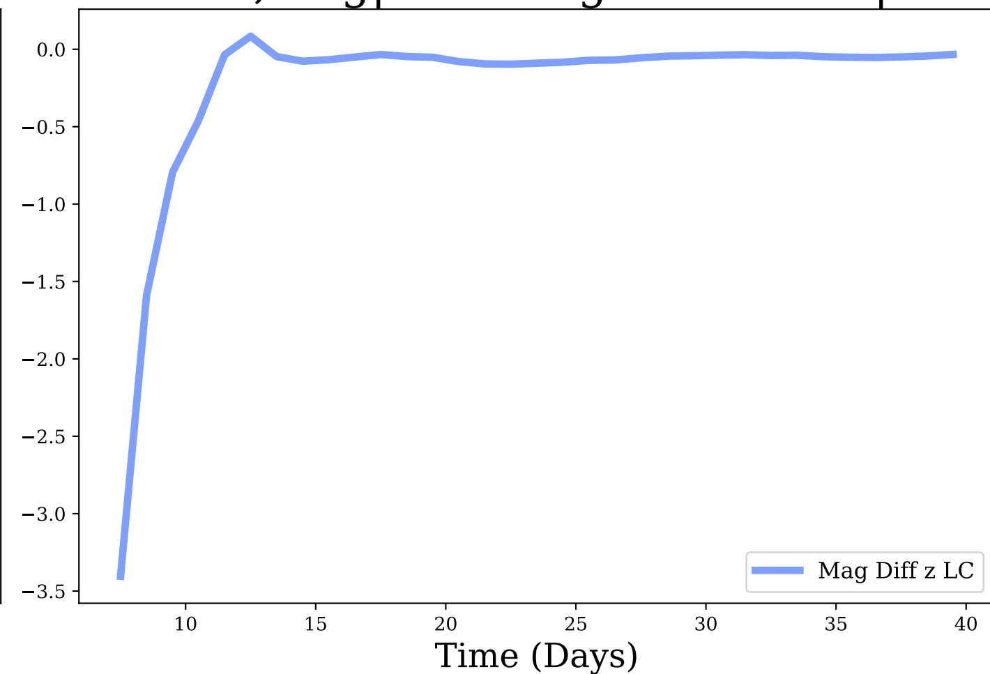
z-band, Avg|Max Mag Diff: -0.23 | 3.4
