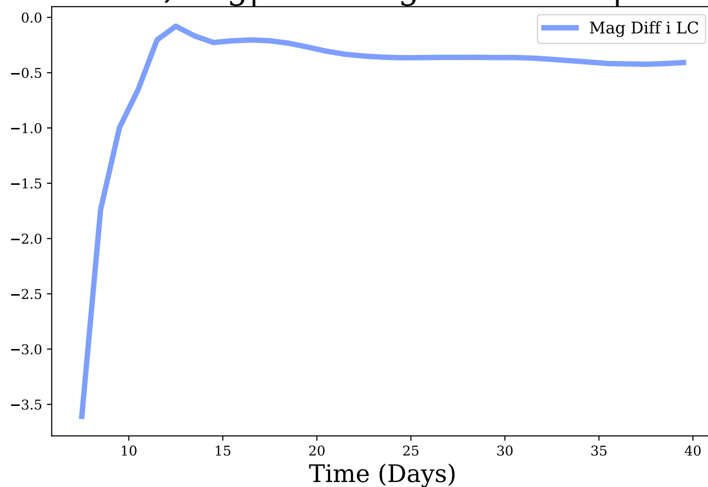
i-band, Avg|Max Mag Diff: -0.49 | 3.61
