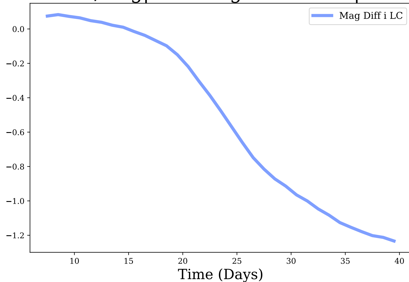
i-band, Avg|Max Mag Diff: -0.52 | 1.23
