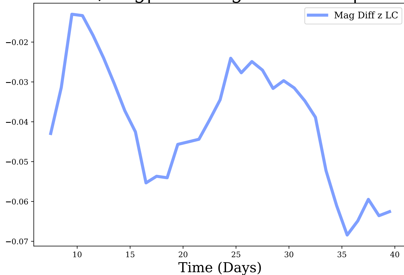
z-band, Avg|Max Mag Diff: -0.04 | 0.07
