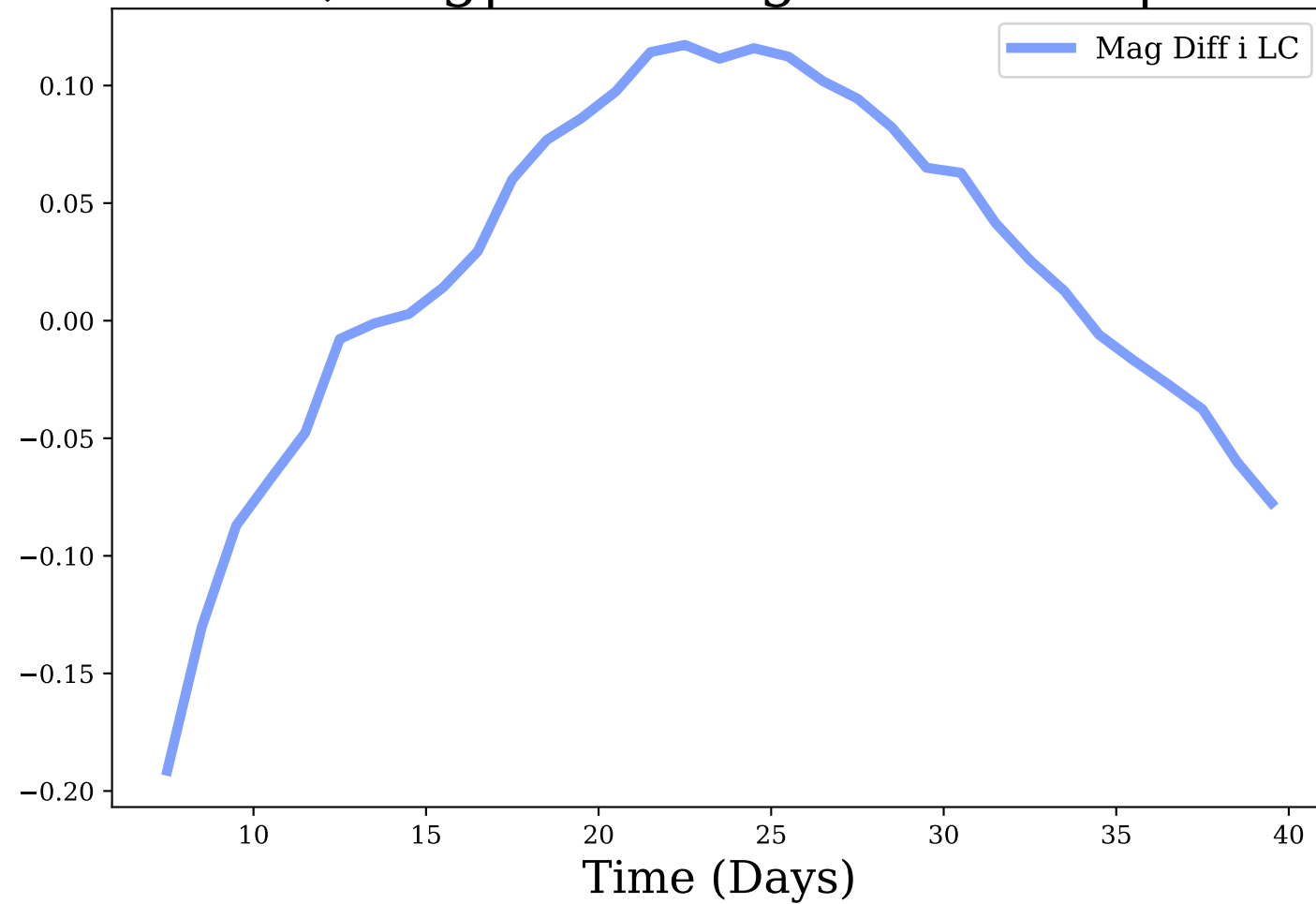
i-band, Avg|Max Mag Diff: 0.02 | 0.19
