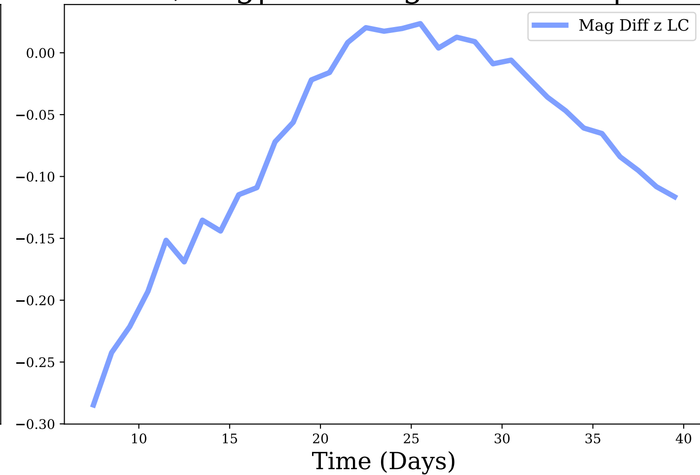
z-band, Avg|Max Mag Diff: -0.07 | 0.28
