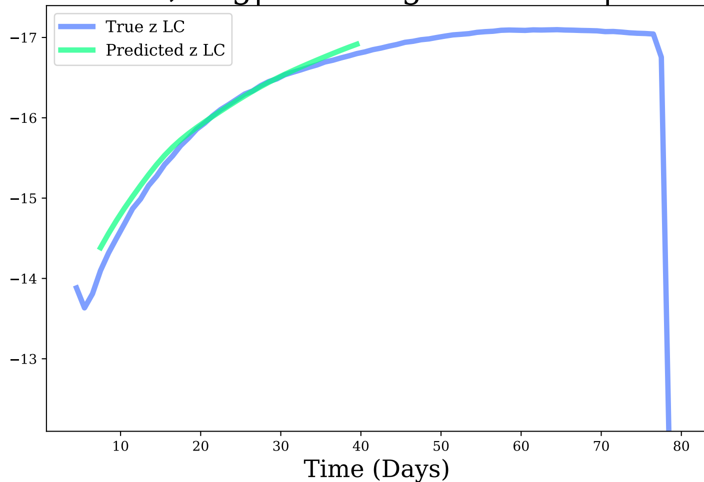
z-band, Avg|Max Mag Diff: 0.08 | 0.28
