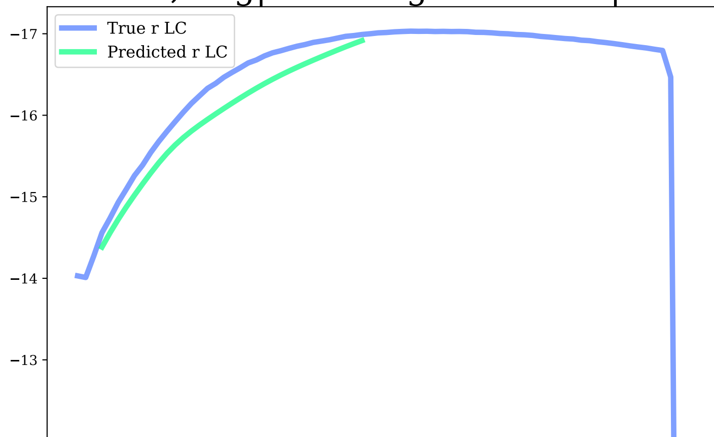
z-band, Avg|Max Mag Diff: 0.08 | 0.28
