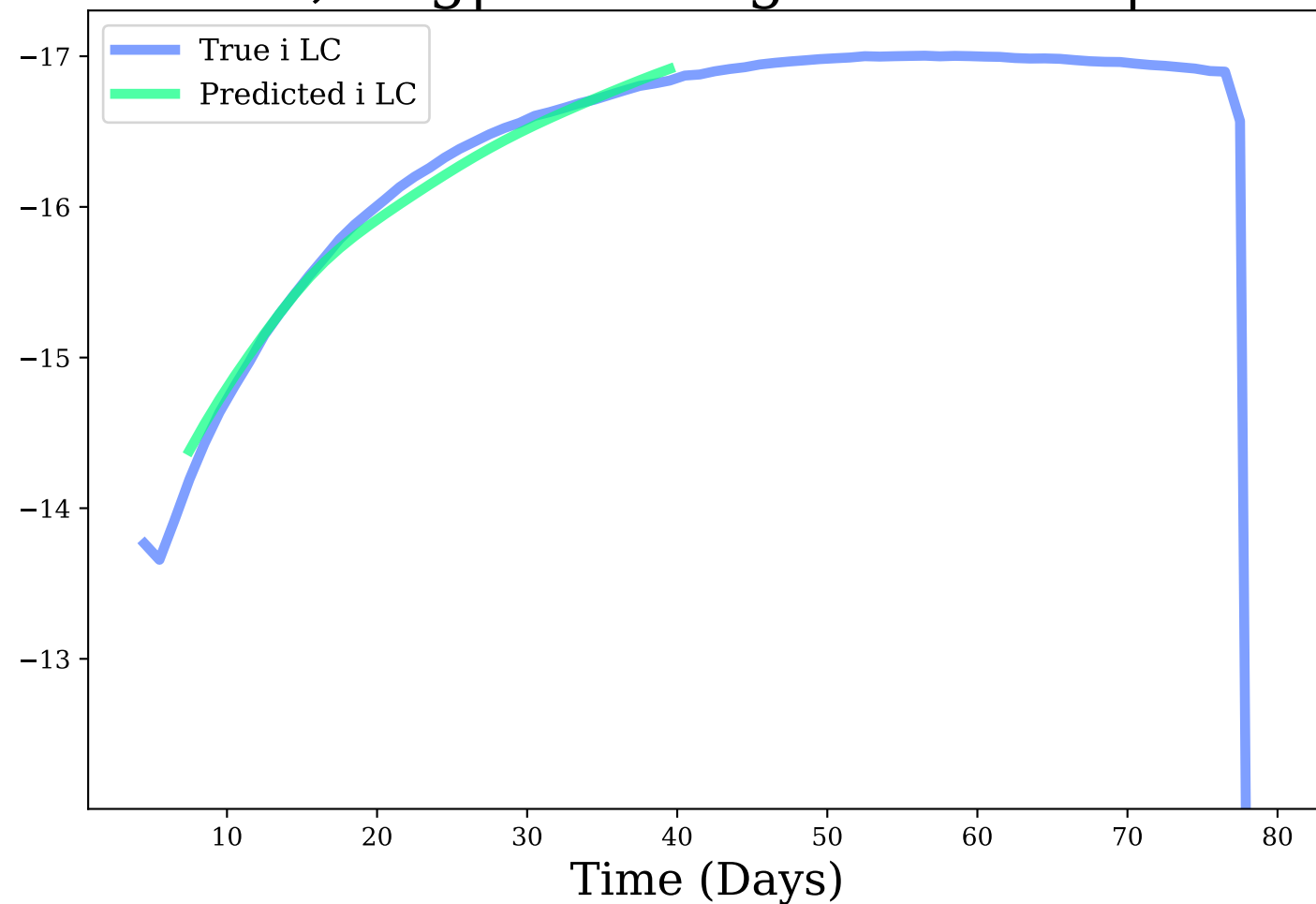
i-band, Avg|Max Mag Diff: 0.07 | 0.19
