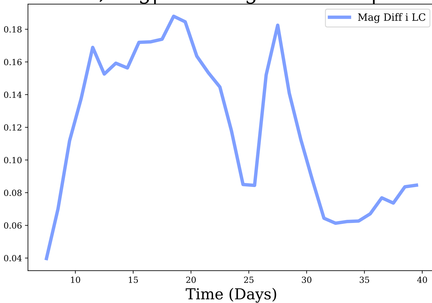
i-band, Avg|Max Mag Diff: 0.12 | 0.19
