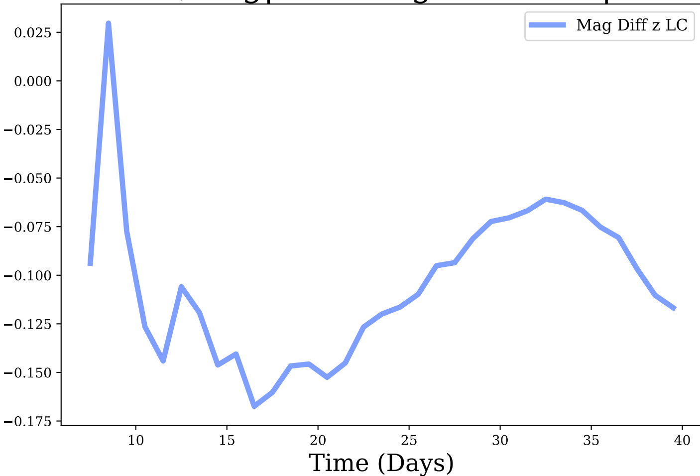
z-band, Avg|Max Mag Diff: -0.1 | 0.17
