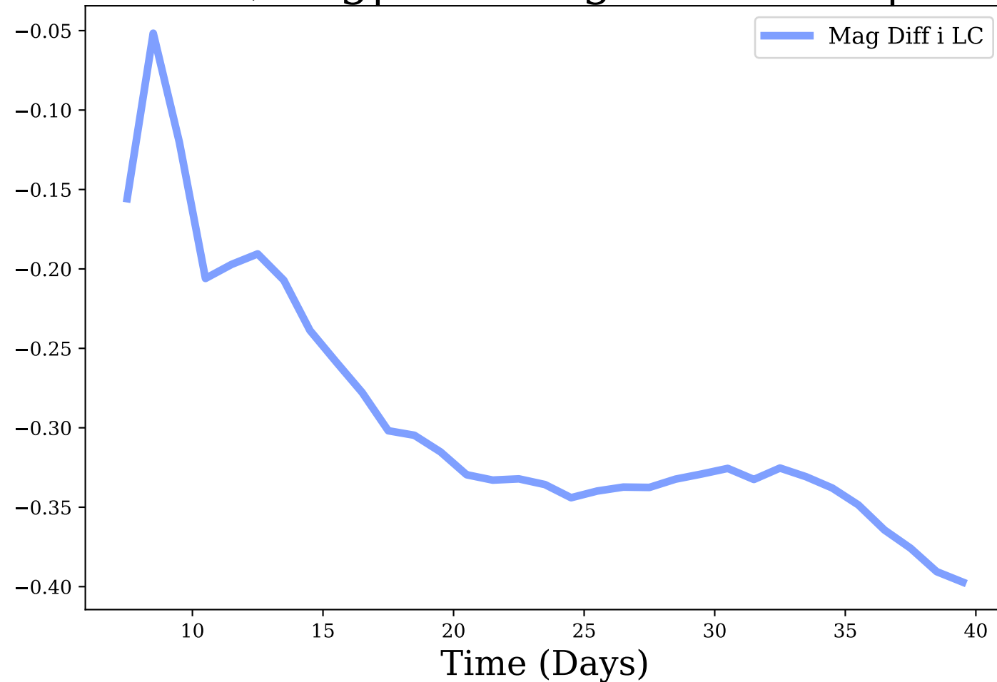
i-band, Avg|Max Mag Diff: -0.29 | 0.4
