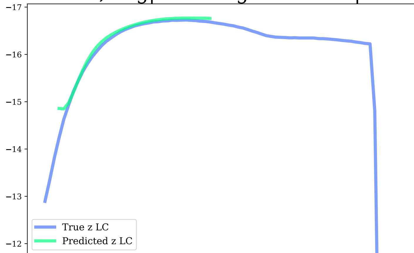
z-band, Avg|Max Mag Diff: 0.07 | 0.62
