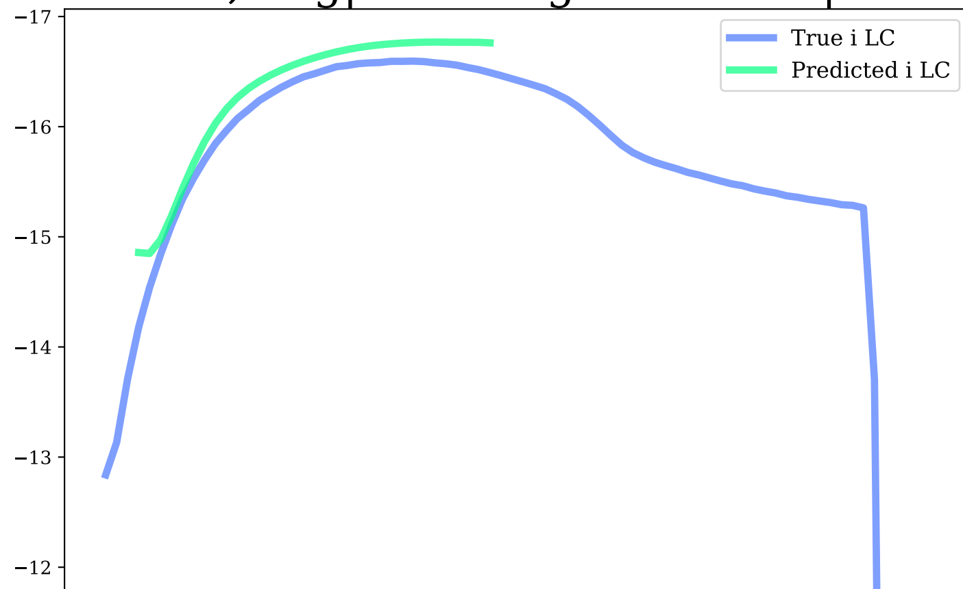
i-band, Avg|Max Mag Diff: 0.19 | 0.68
