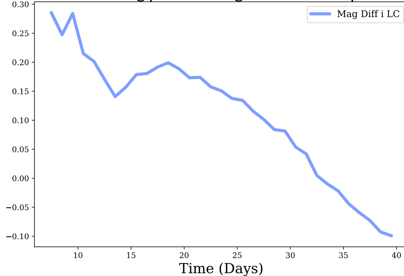
i-band, Avg|Max Mag Diff: 0.11 | 0.29
