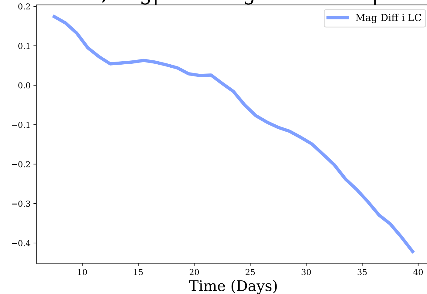
i-band, Avg|Max Mag Diff: -0.07 | 0.42
