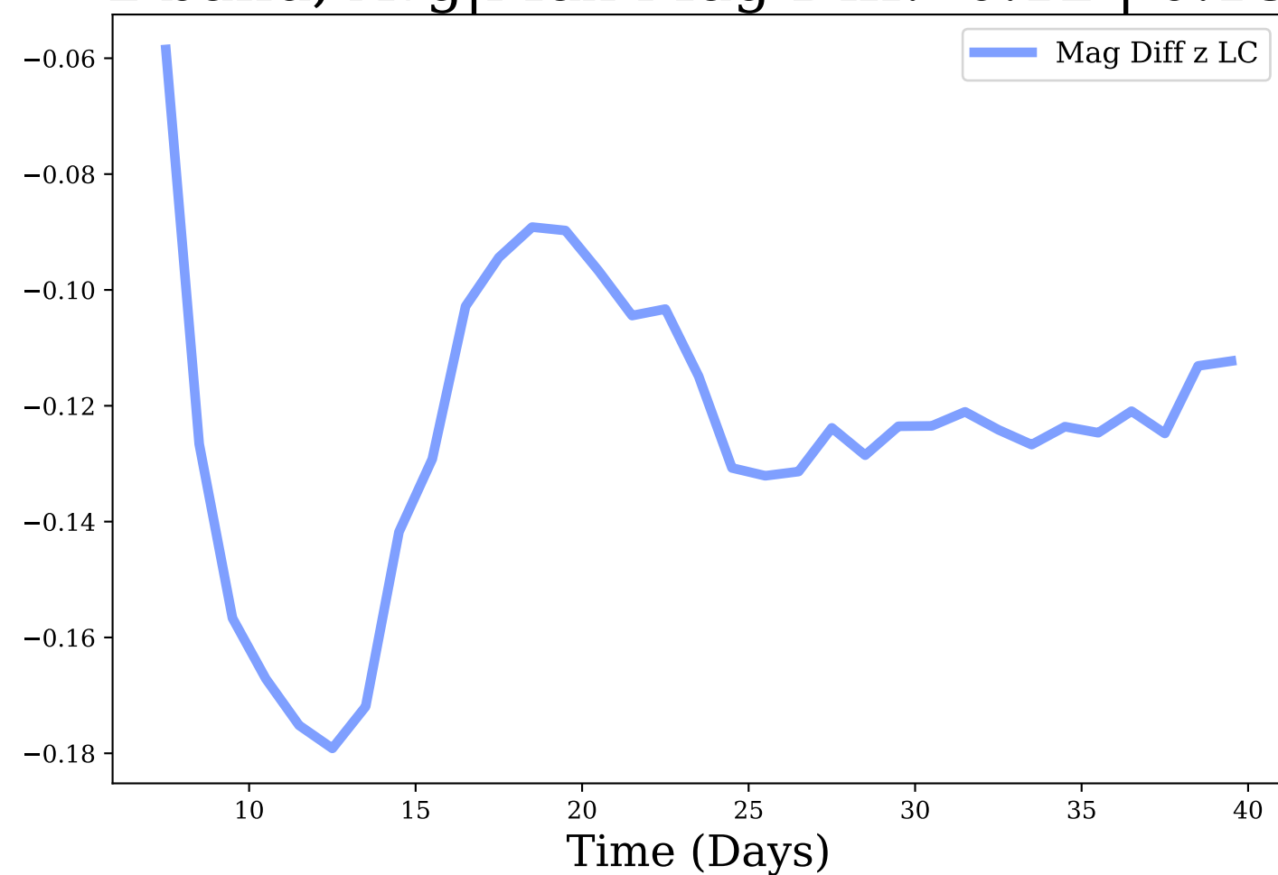
z-band, Avg|Max Mag Diff: -0.12 | 0.18
