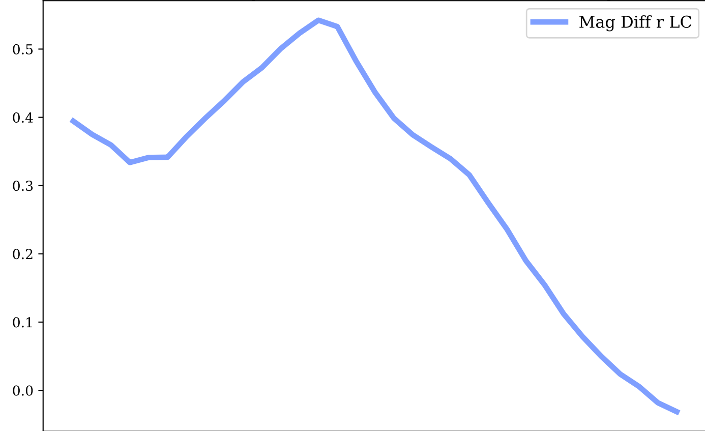
r-band, Avg|Max Mag Diff: 0.31 | 0.54
