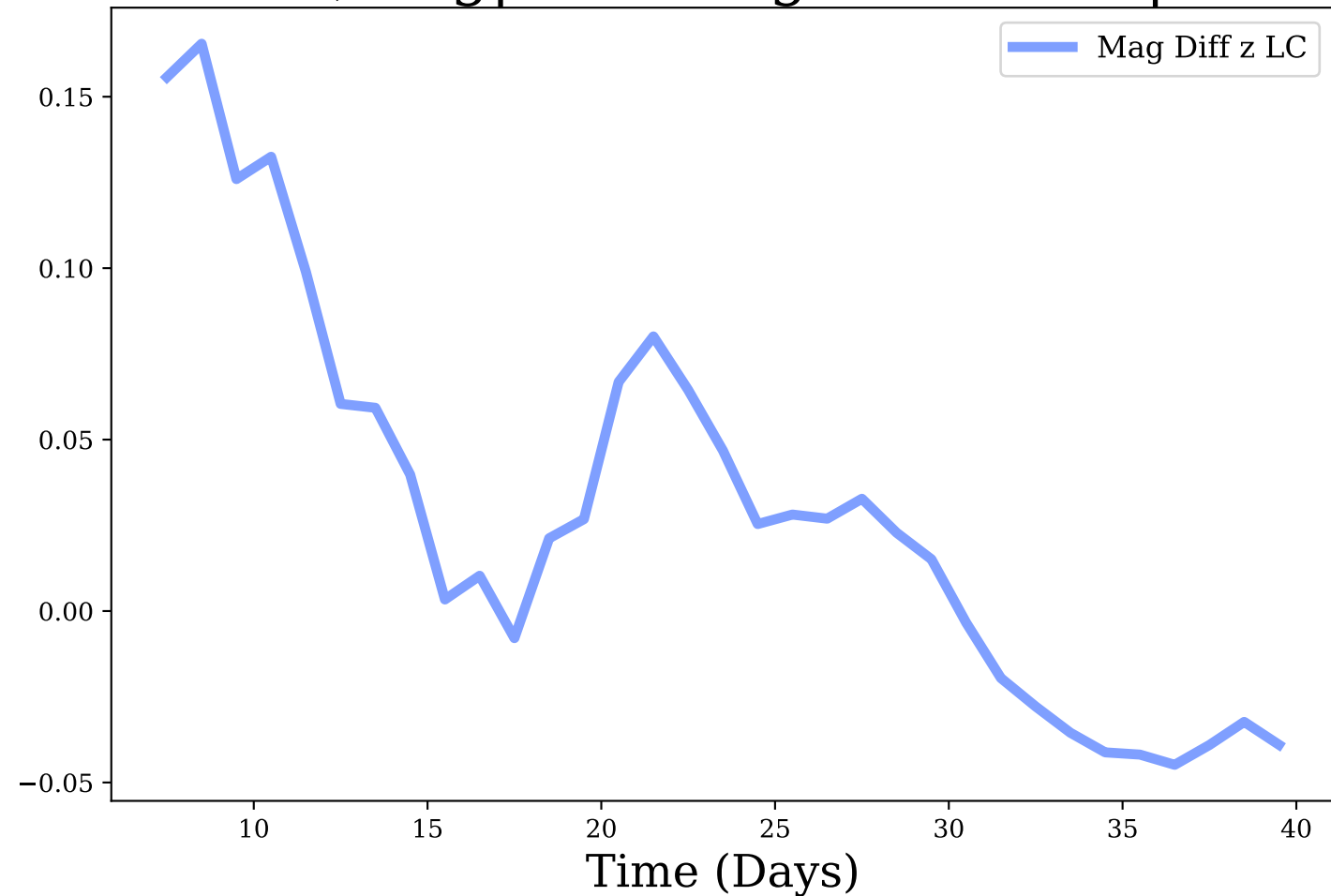
z-band, Avg|Max Mag Diff: 0.03 | 0.17
