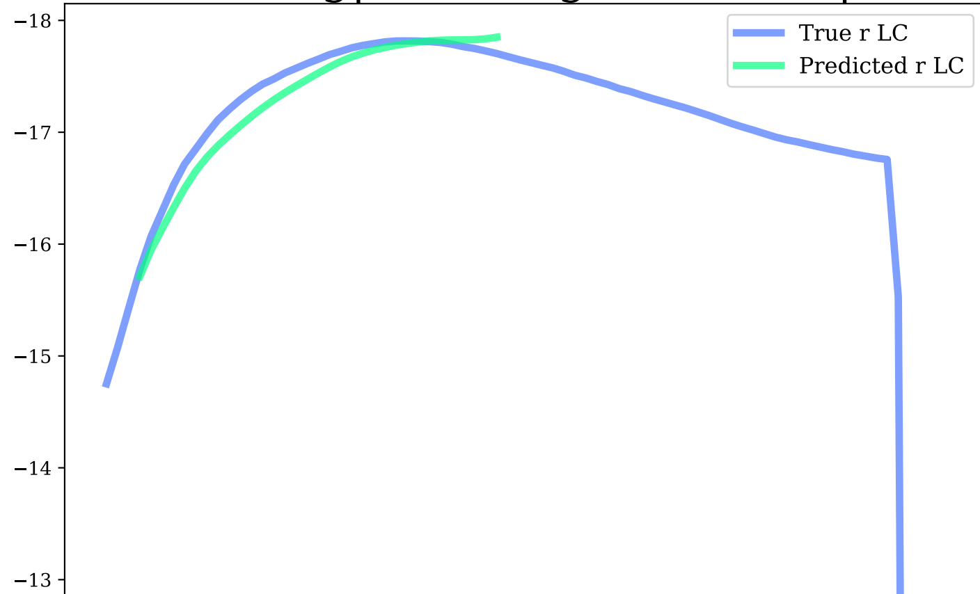
z-band, Avg|Max Mag Diff: 0.13 | 0.19
