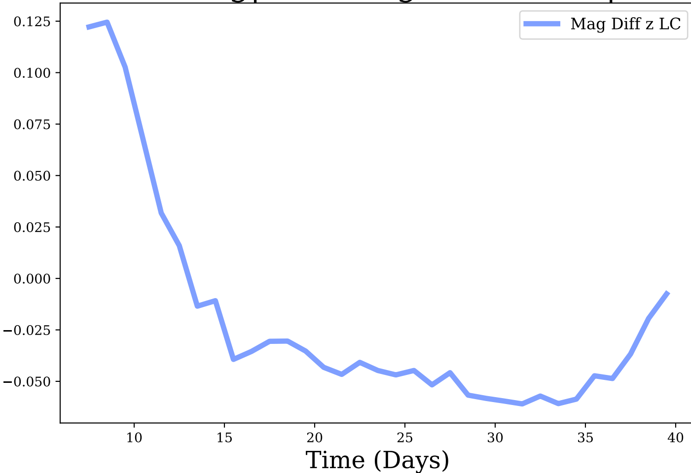
z-band, Avg|Max Mag Diff: -0.02 | 0.12
