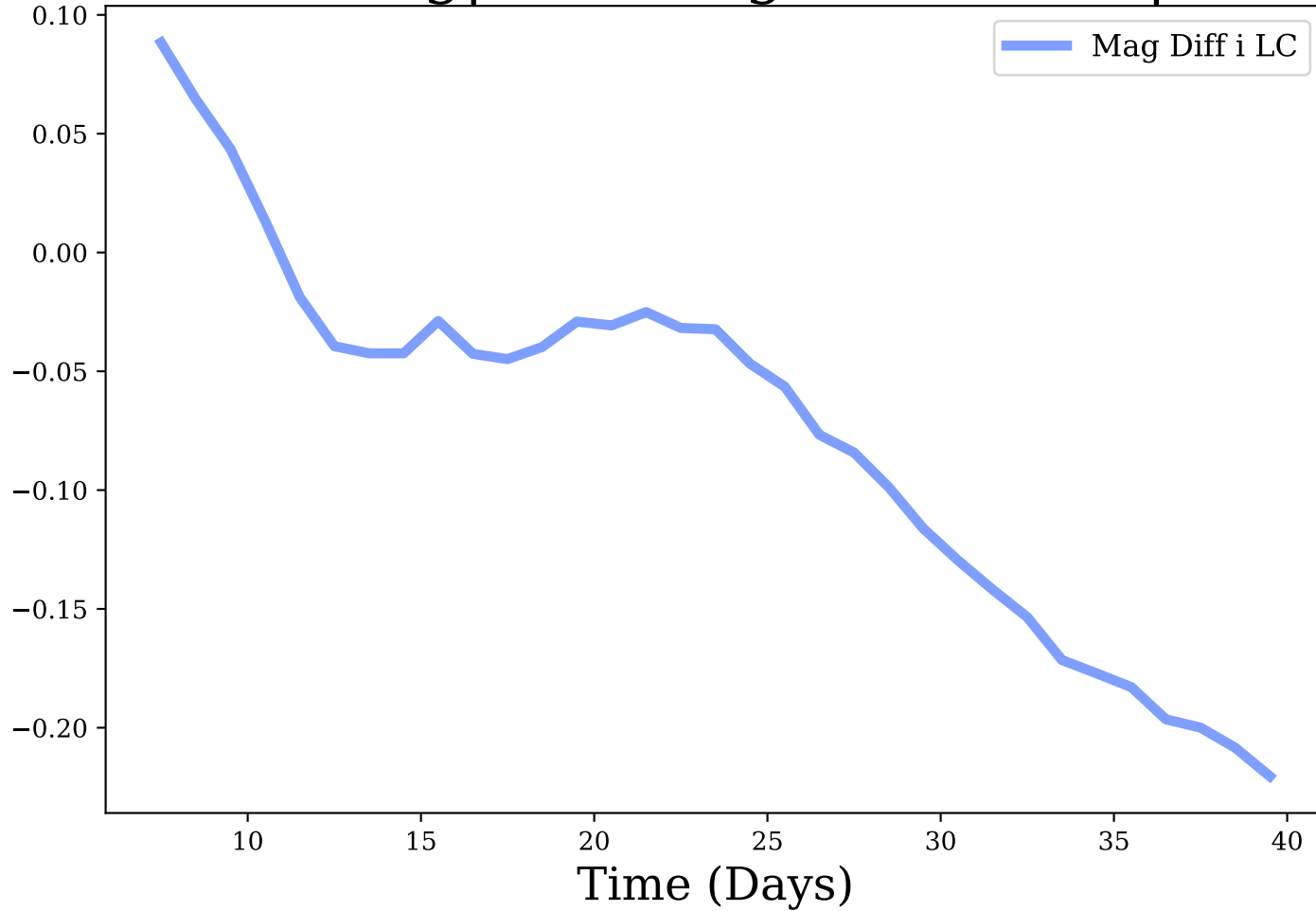
i-band, Avg|Max Mag Diff: -0.08 | 0.22
