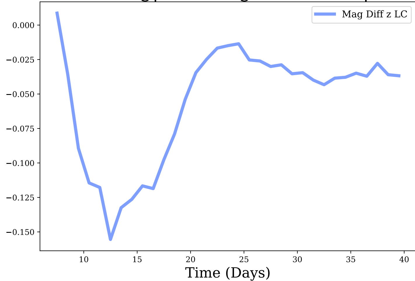
z-band, Avg|Max Mag Diff: -0.06 | 0.16
