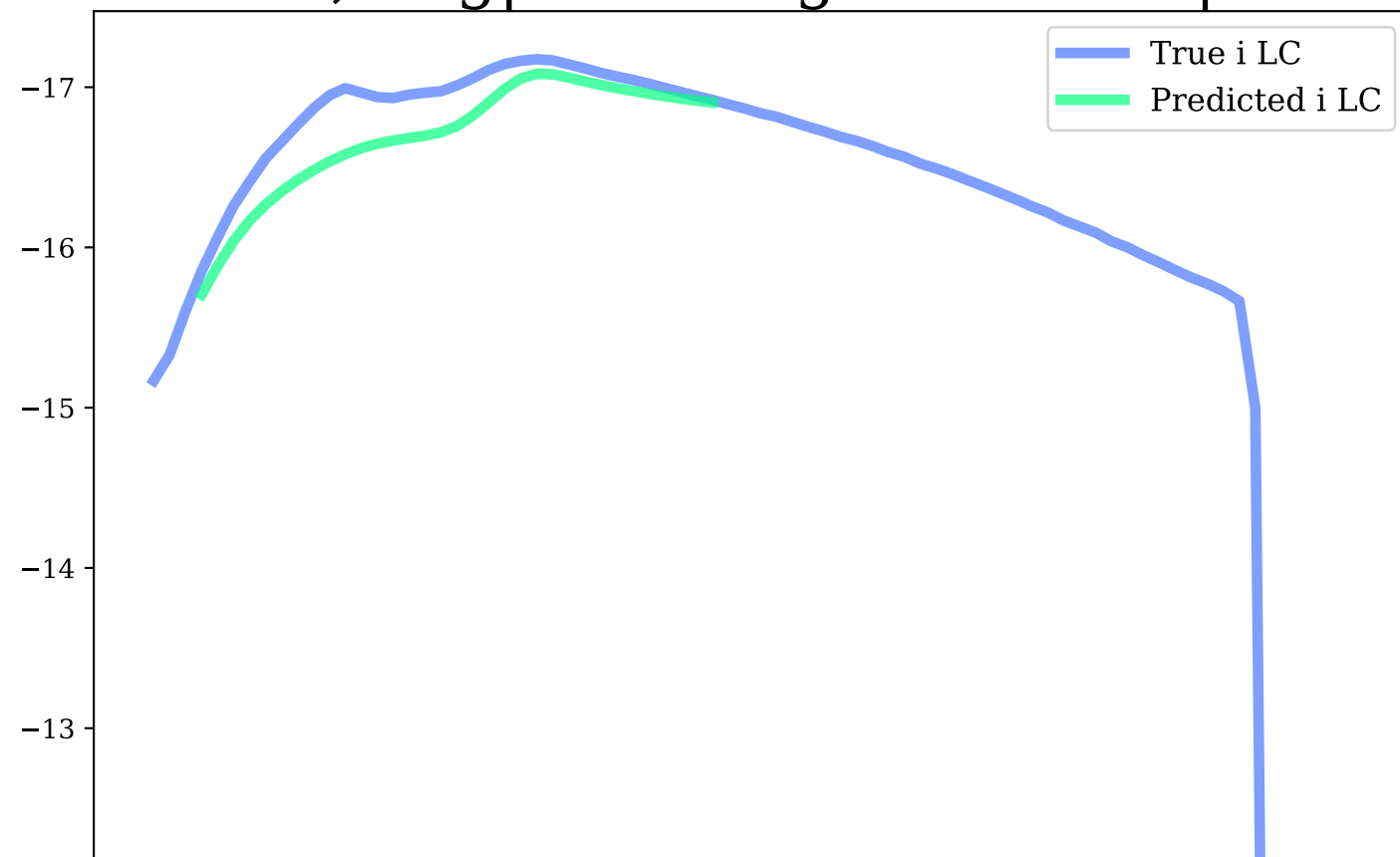
i-band, Avg|Max Mag Diff: 0.19 | 0.41
