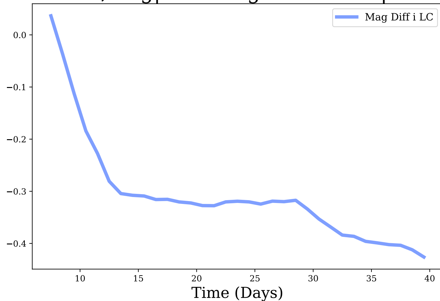
i-band, Avg|Max Mag Diff: -0.31 | 0.43
