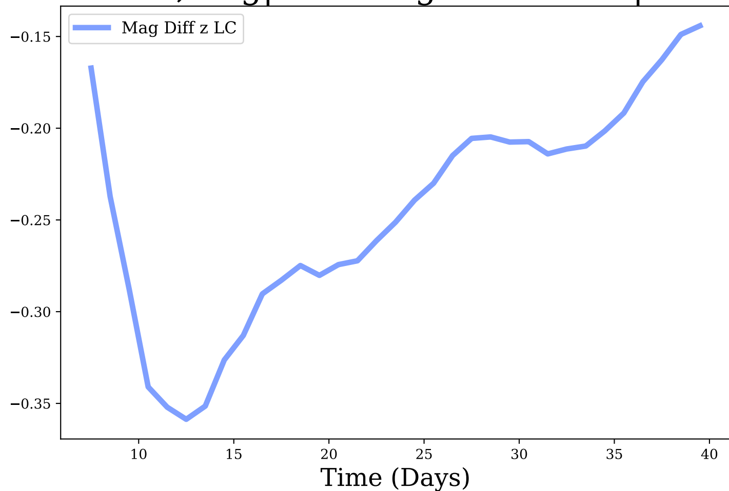
z-band, Avg|Max Mag Diff: -0.25 | 0.36
