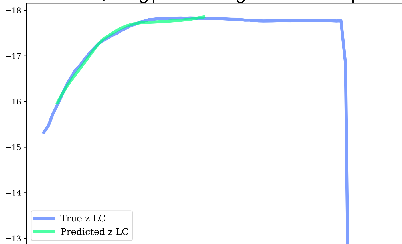
z-band, Avg|Max Mag Diff: 0.04 | 0.1
