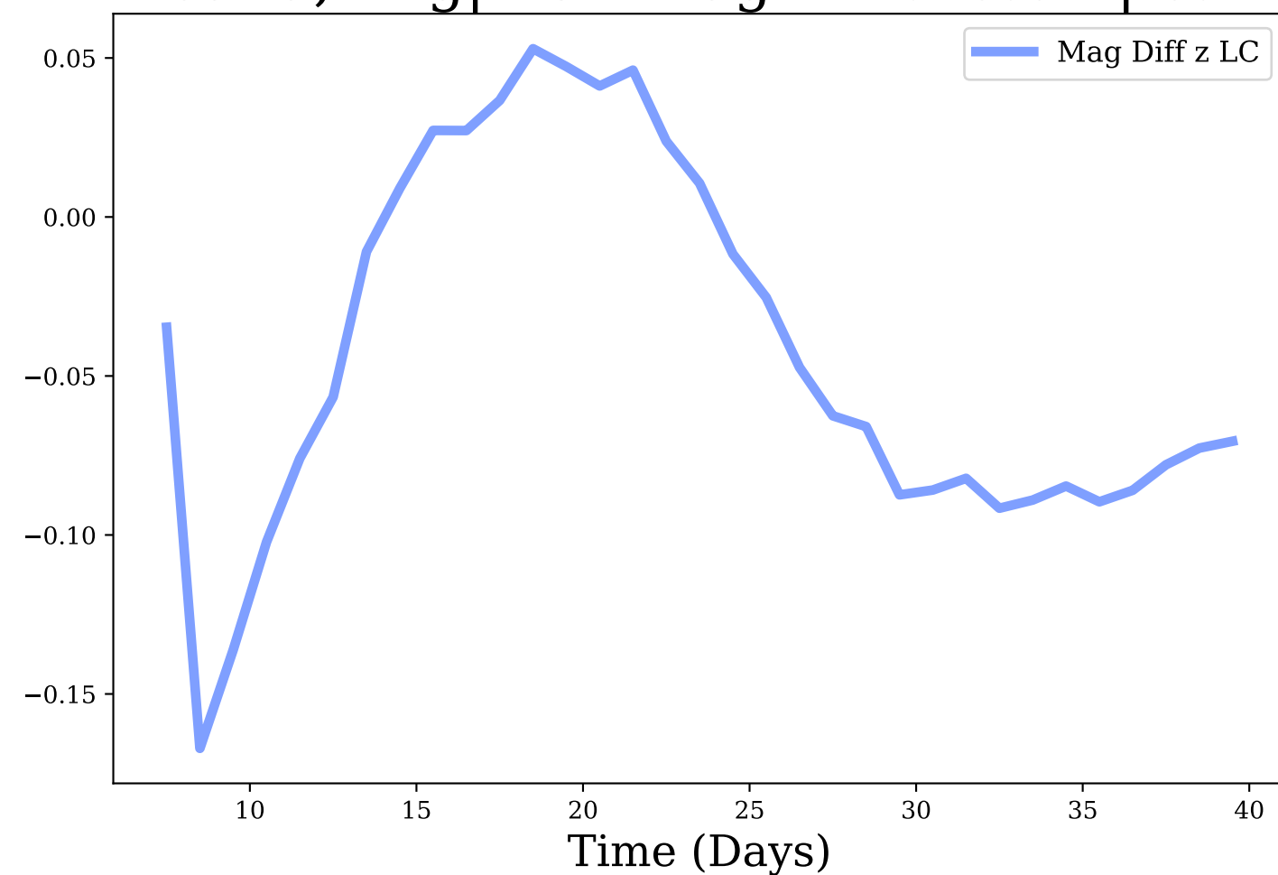
z-band, Avg|Max Mag Diff: -0.04 | 0.17
