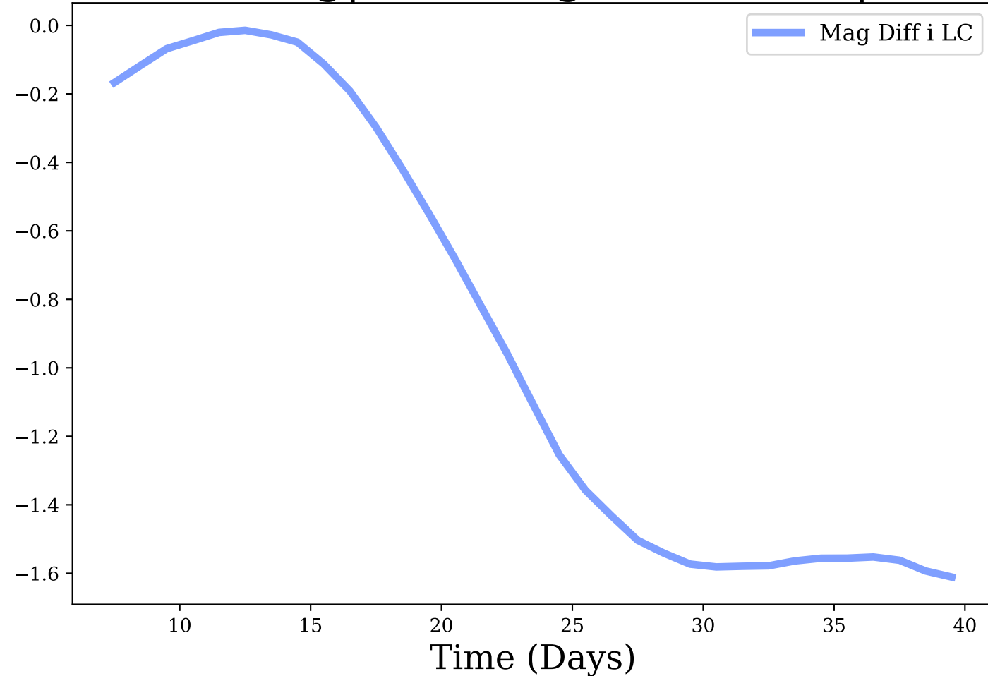
i-band, Avg|Max Mag Diff: -0.91 | 1.61
