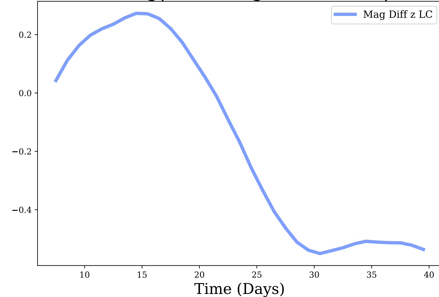
z-band, Avg|Max Mag Diff: -0.16 | 0.55
