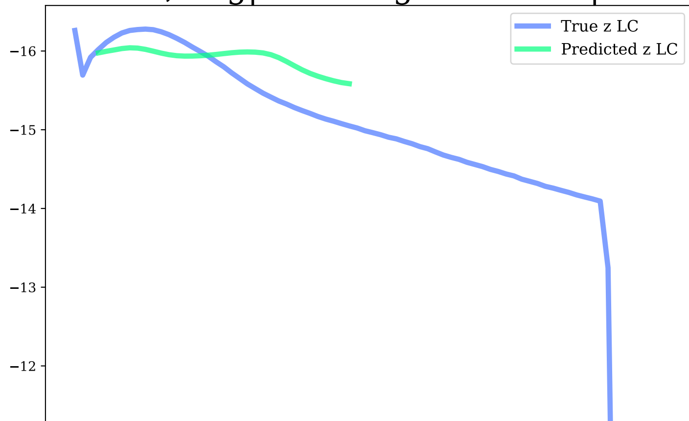
z-band, Avg|Max Mag Diff: 0.32 | 0.55
