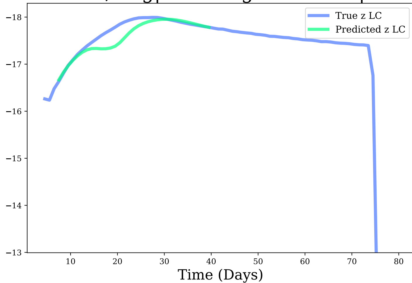
z-band, Avg|Max Mag Diff: 0.12 | 0.4
