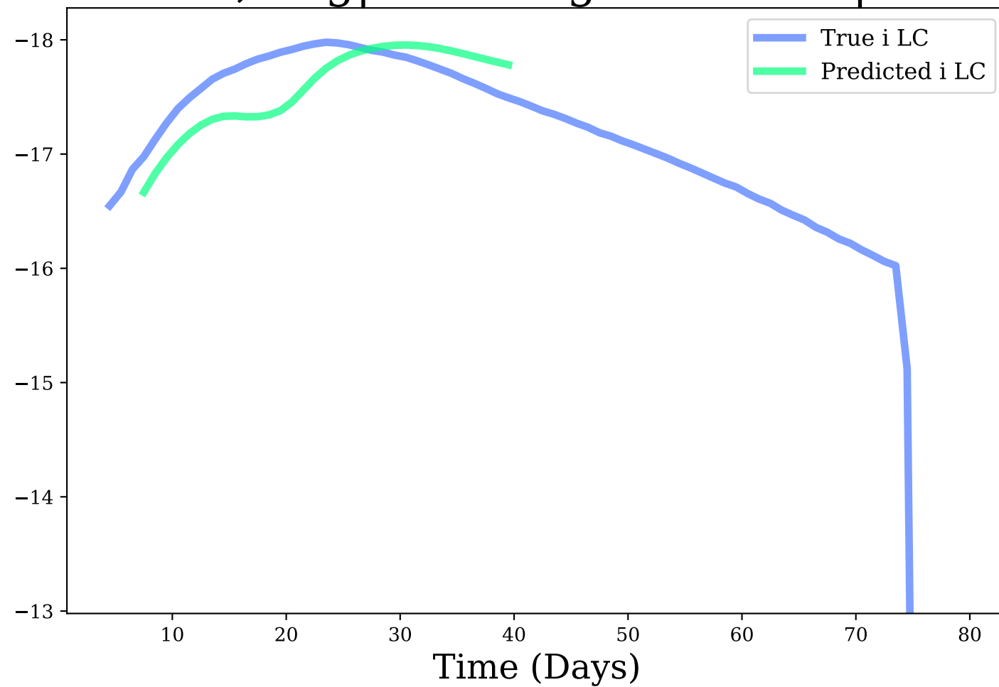
i-band, Avg|Max Mag Diff: 0.27 | 0.52
