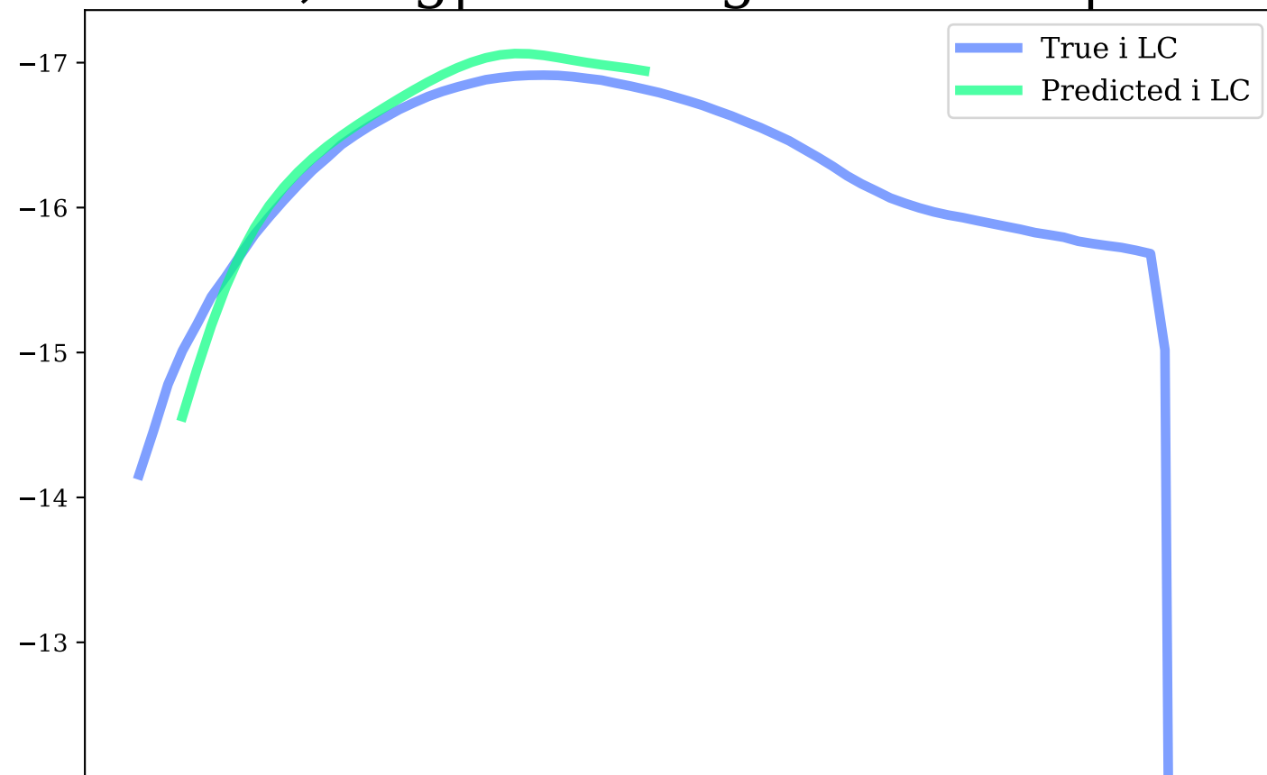
i-band, Avg|Max Mag Diff: 0.12 | 0.45
