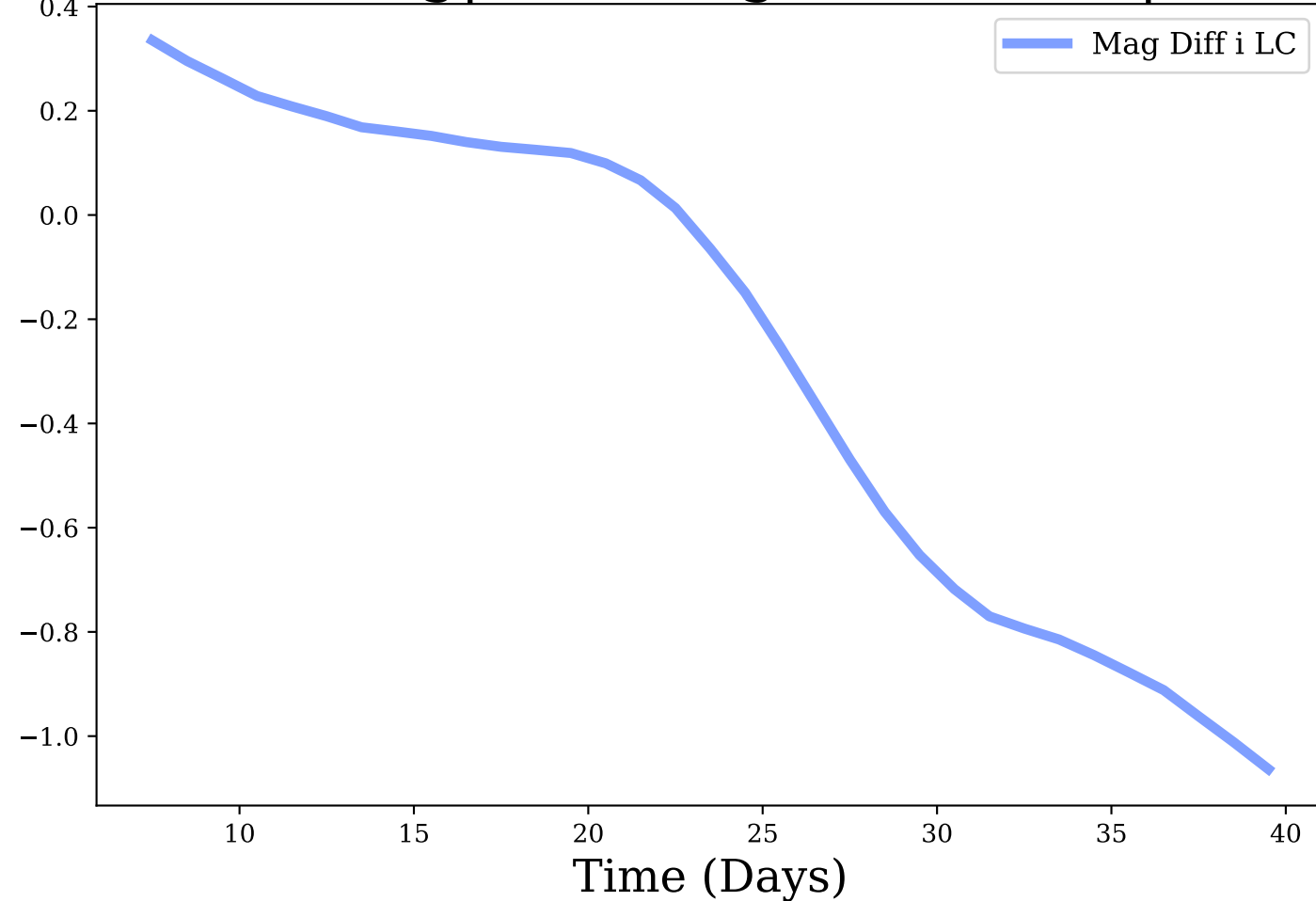
i-band, Avg|Max Mag Diff: -0.26 | 1.06
