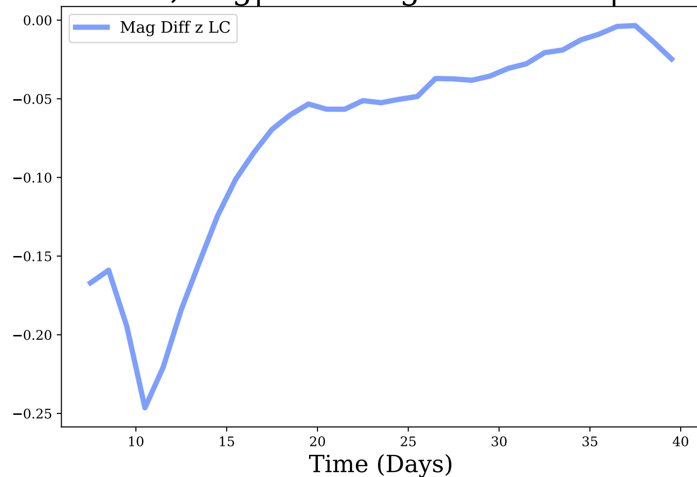
z-band, Avg|Max Mag Diff: -0.07 | 0.25
