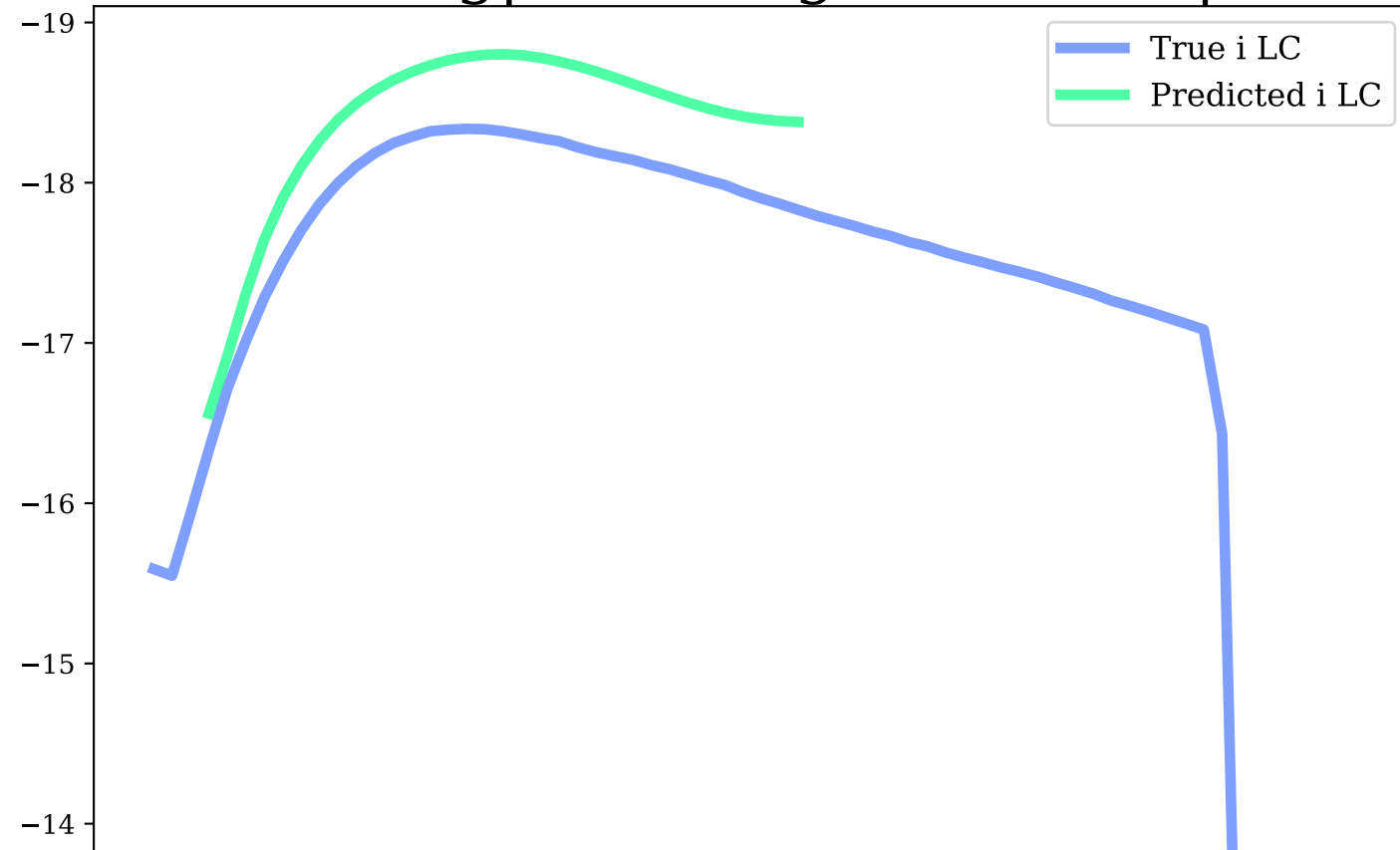
i-band, Avg|Max Mag Diff: 0.43 | 0.55
