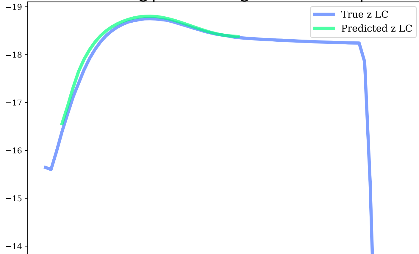
z-band, Avg|Max Mag Diff: 0.07 | 0.25
