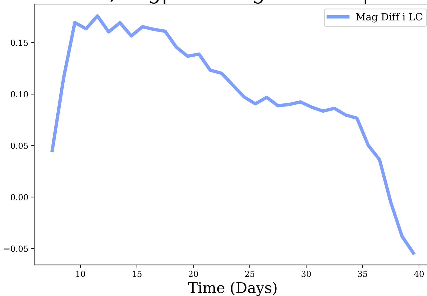
i-band, Avg|Max Mag Diff: 0.1 | 0.18
