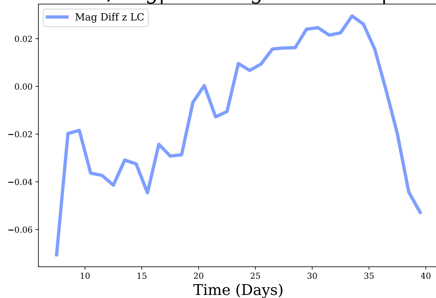
z-band, Avg|Max Mag Diff: -0.01 | 0.07
