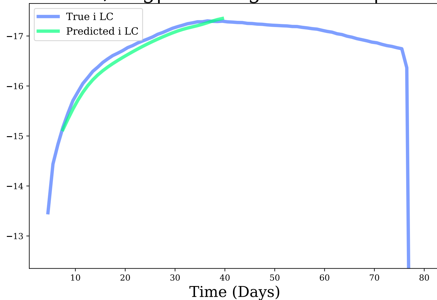
i-band, Avg|Max Mag Diff: 0.11 | 0.18
