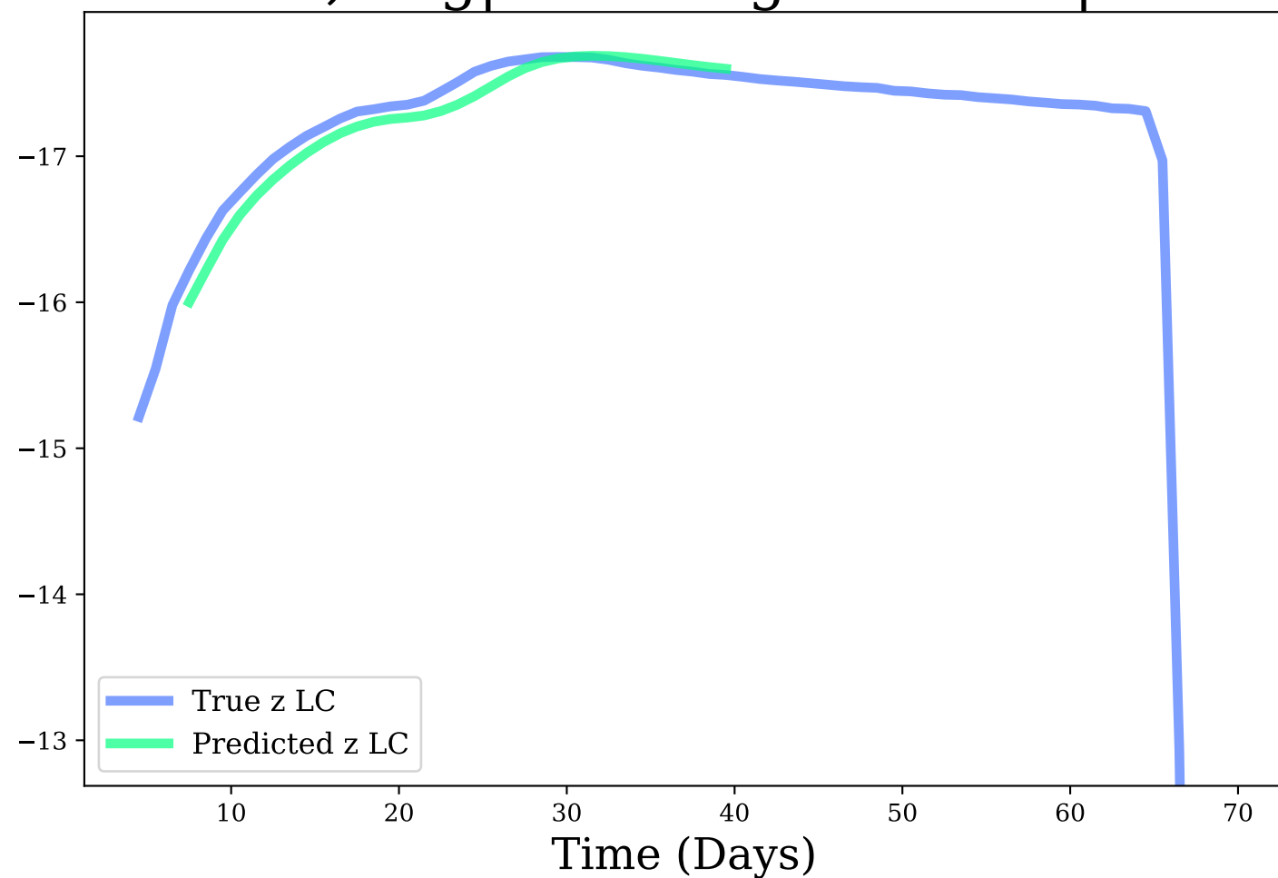
z-band, Avg|Max Mag Diff: 0.1 | 0.22
