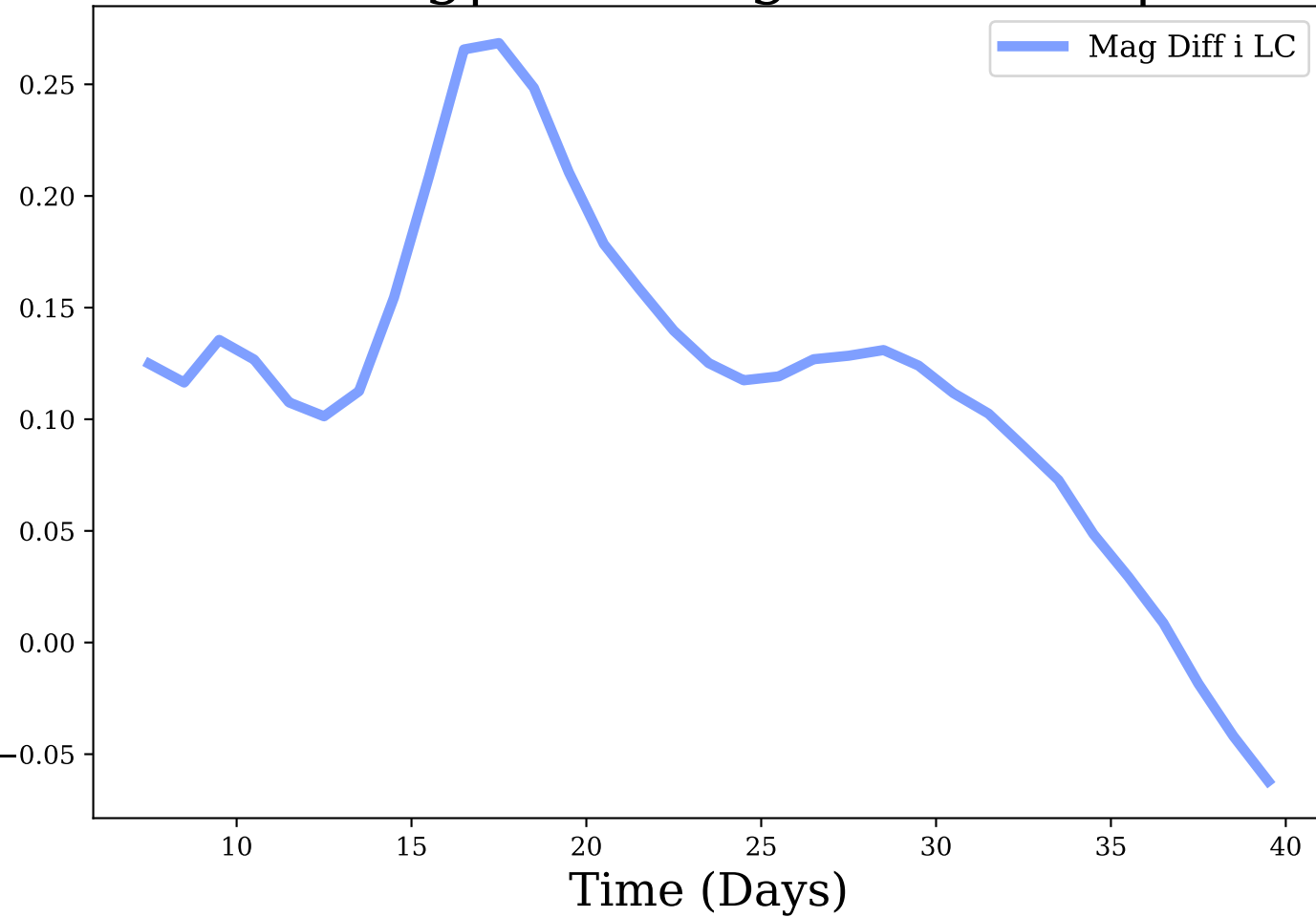
i-band, Avg|Max Mag Diff: 0.12 | 0.27
