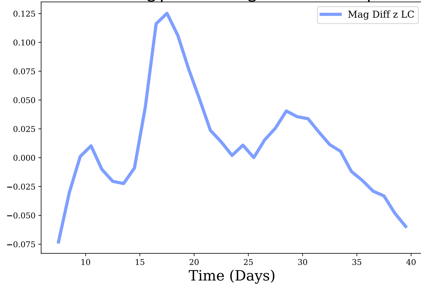
z-band, Avg|Max Mag Diff: 0.01 | 0.13
