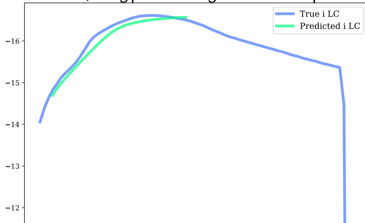
i-band, Avg|Max Mag Diff: 0.12 | 0.27
