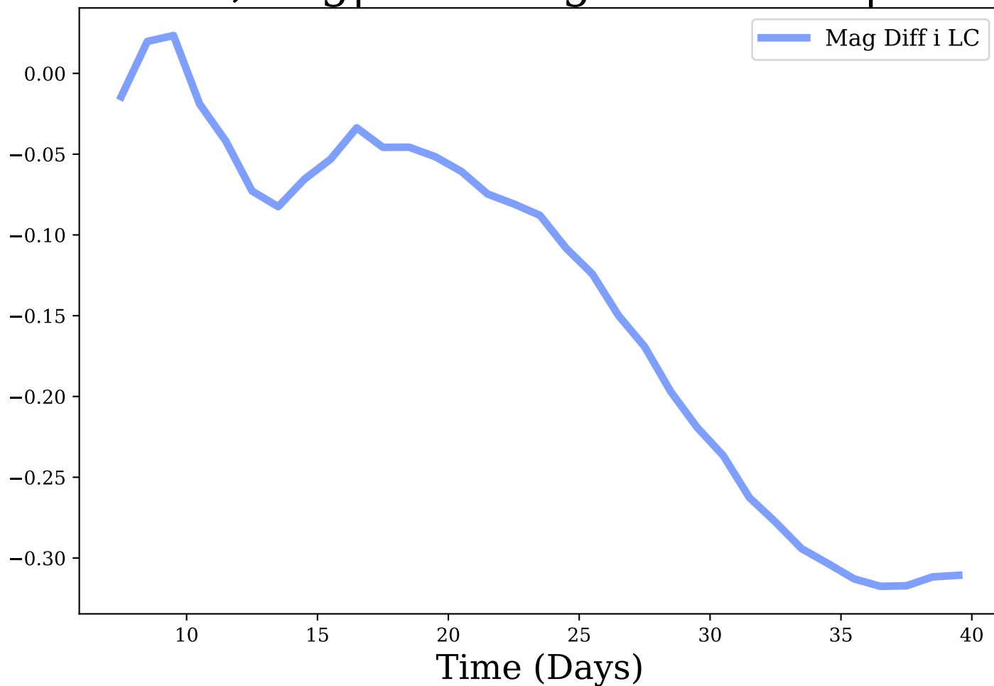
i-band, Avg|Max Mag Diff: -0.14 | 0.32
