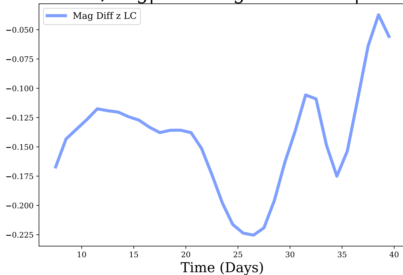
z-band, Avg|Max Mag Diff: -0.14 | 0.23
