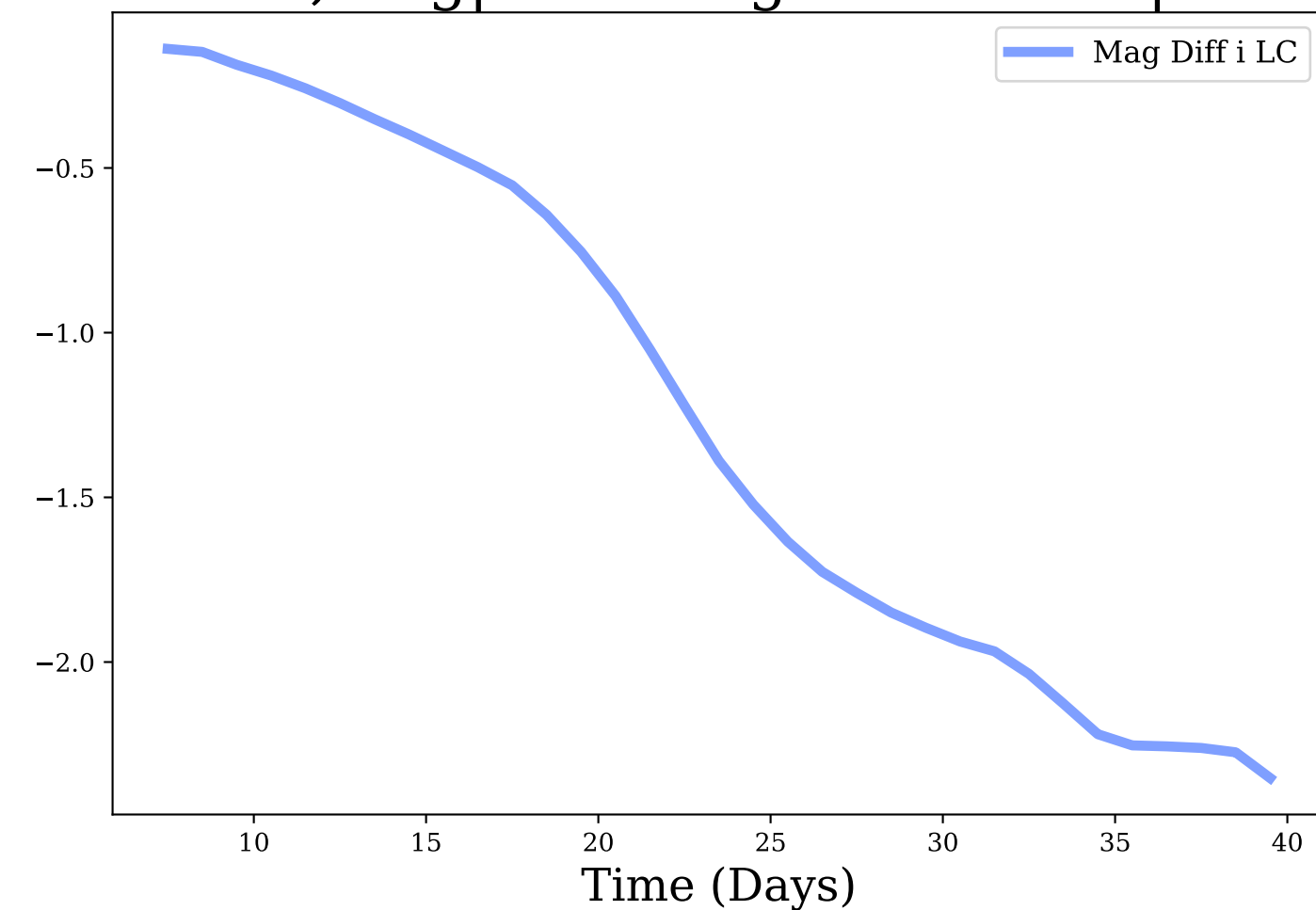
i-band, Avg|Max Mag Diff: -1.26 | 2.35
