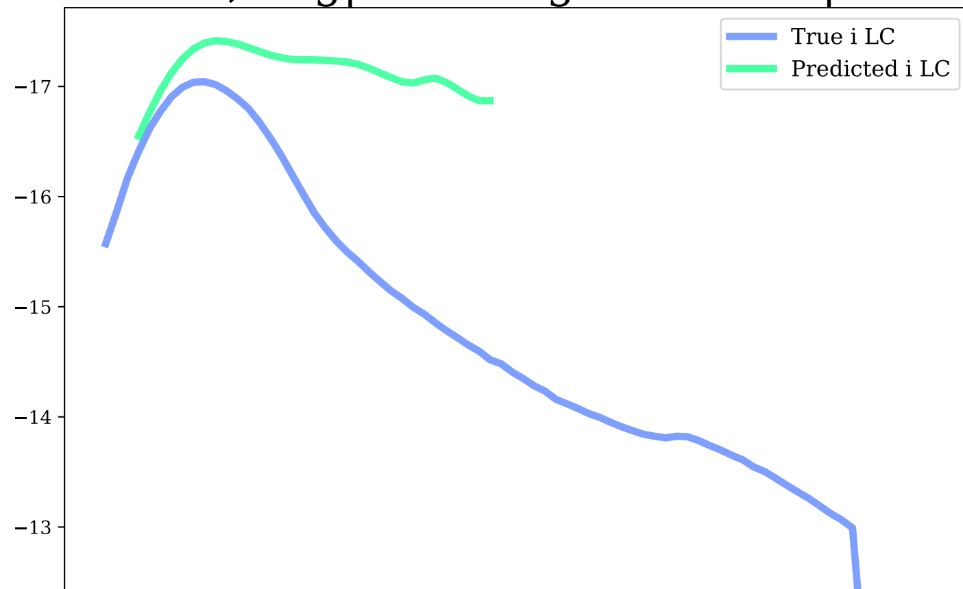
i-band, Avg|Max Mag Diff: 1.26 | 2.35
