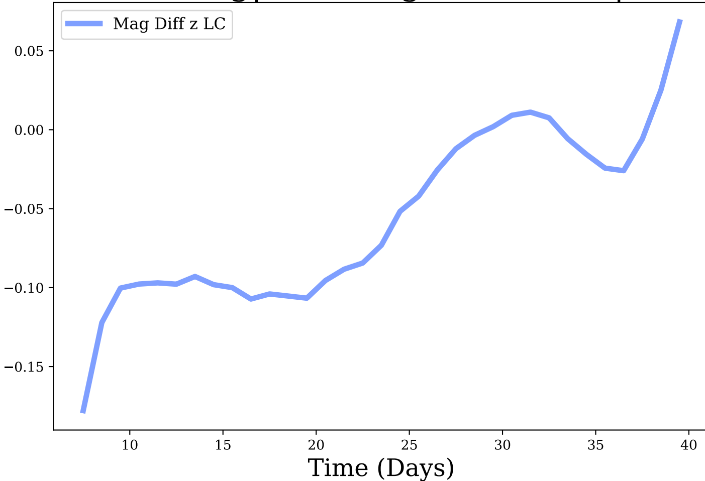
z-band, Avg|Max Mag Diff: -0.06 | 0.18
