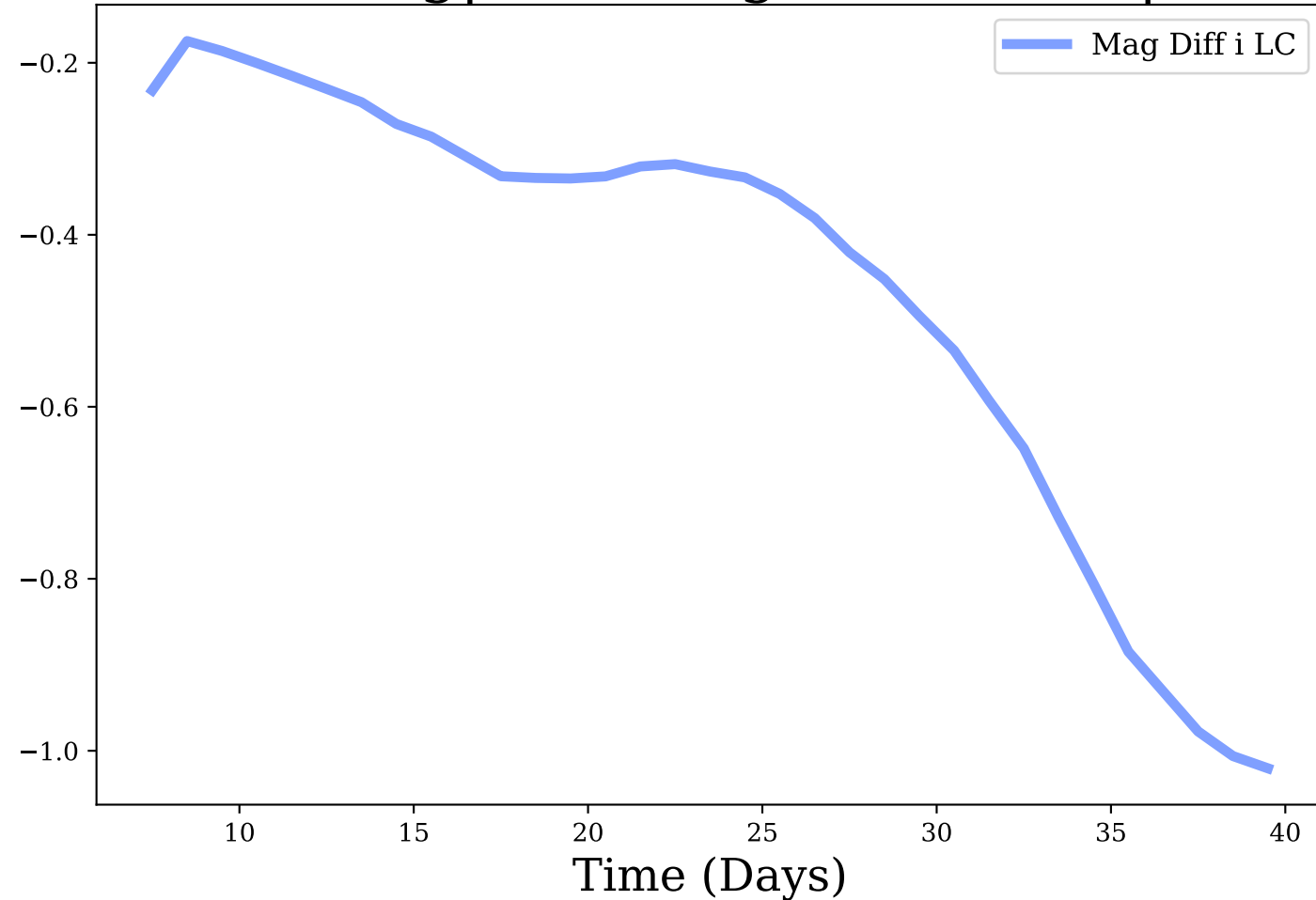
i-band, Avg|Max Mag Diff: -0.46 | 1.02
