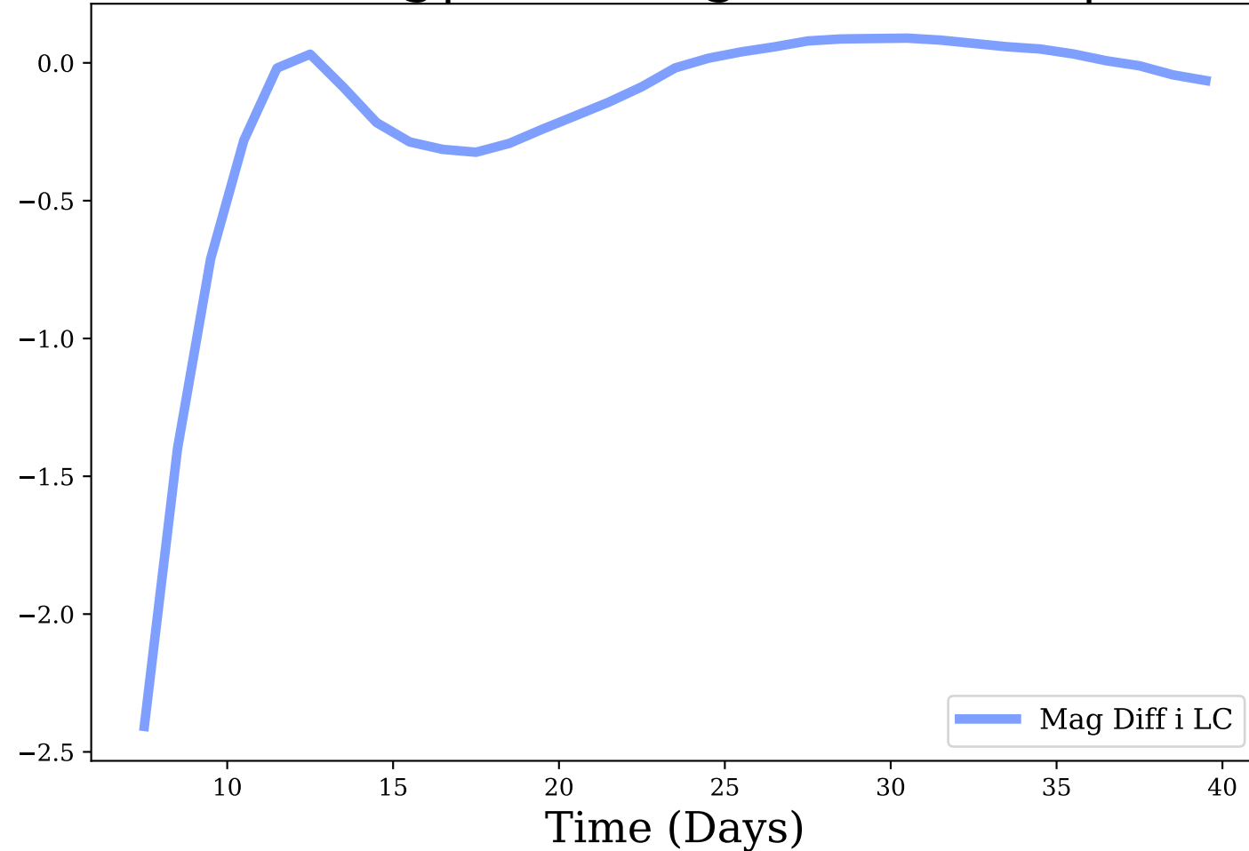
i-band, Avg|Max Mag Diff: -0.19 | 2.41
