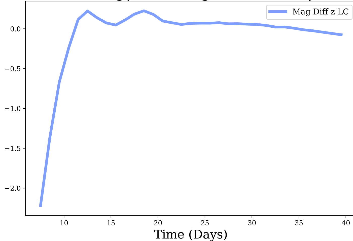
z-band, Avg|Max Mag Diff: -0.08 | 2.22
