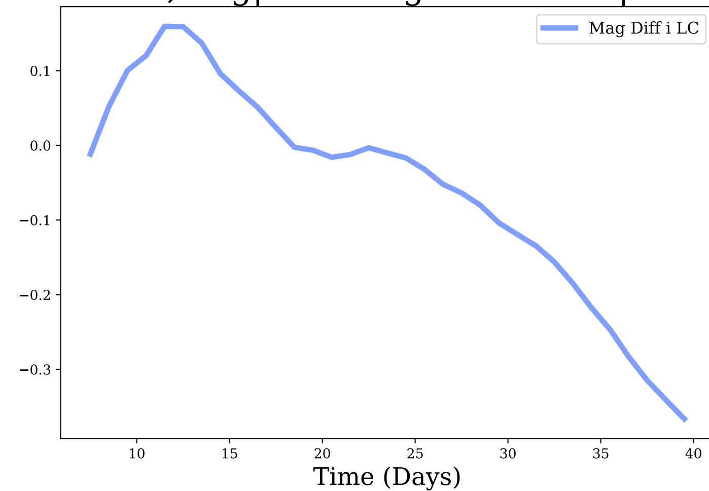
i-band, Avg|Max Mag Diff: -0.05 | 0.37
