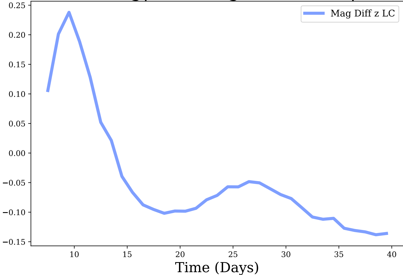
z-band, Avg|Max Mag Diff: -0.04 | 0.24
