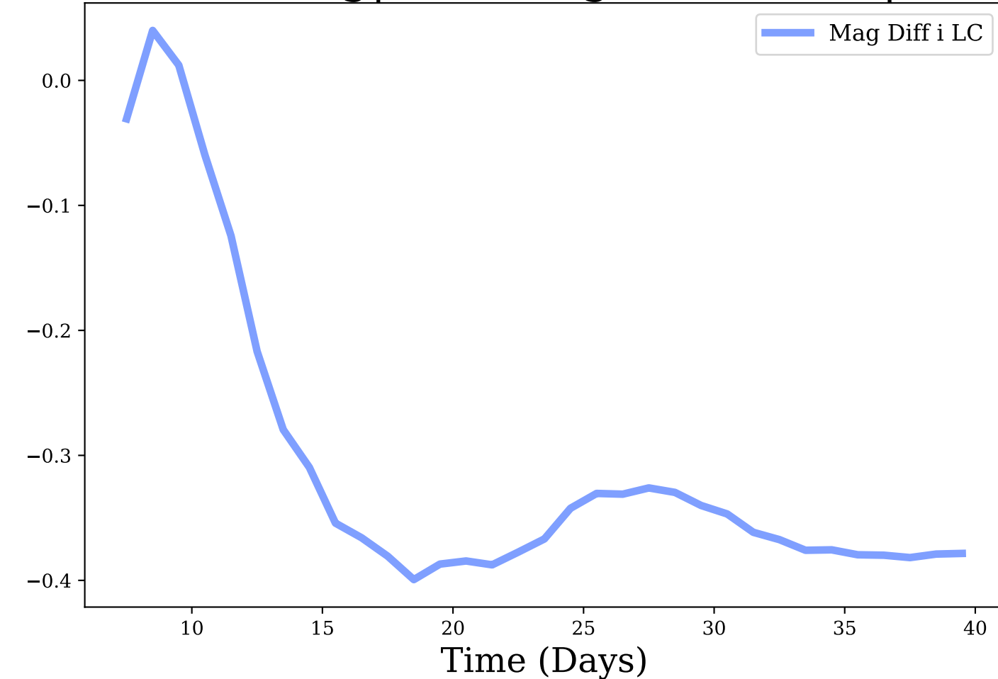
i-band, Avg|Max Mag Diff: -0.31 | 0.4
