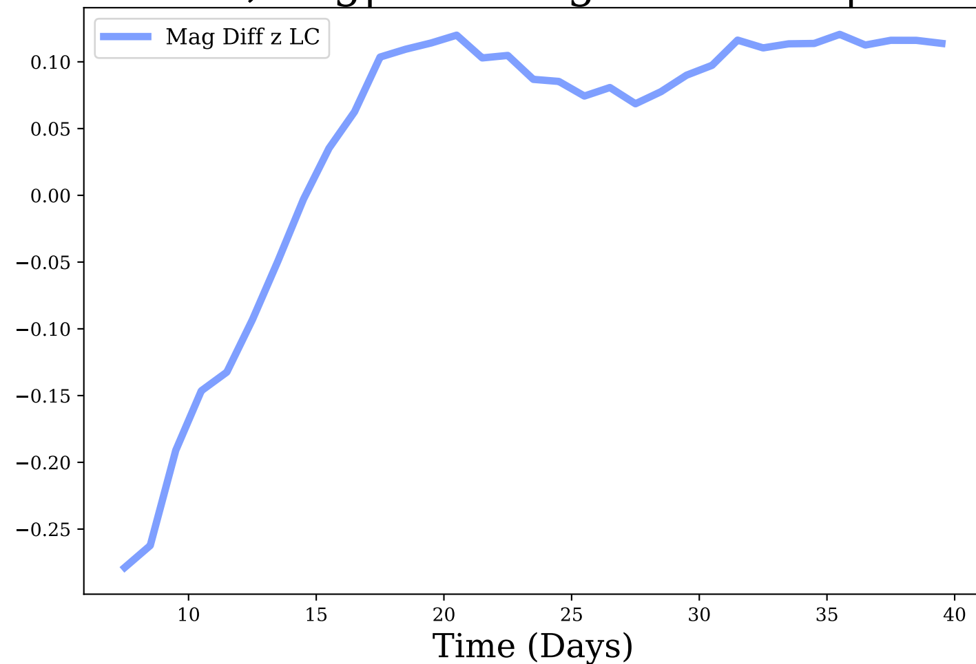
z-band, Avg|Max Mag Diff: 0.04 | 0.28
