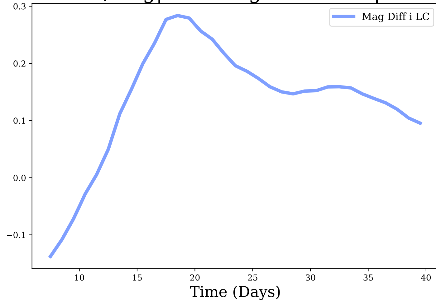
i-band, Avg|Max Mag Diff: 0.14 | 0.28
