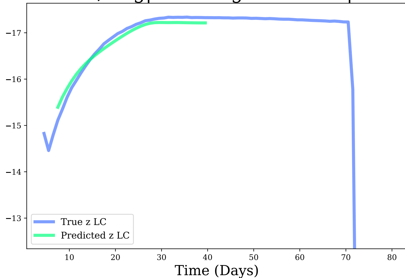
z-band, Avg|Max Mag Diff: 0.11 | 0.28
