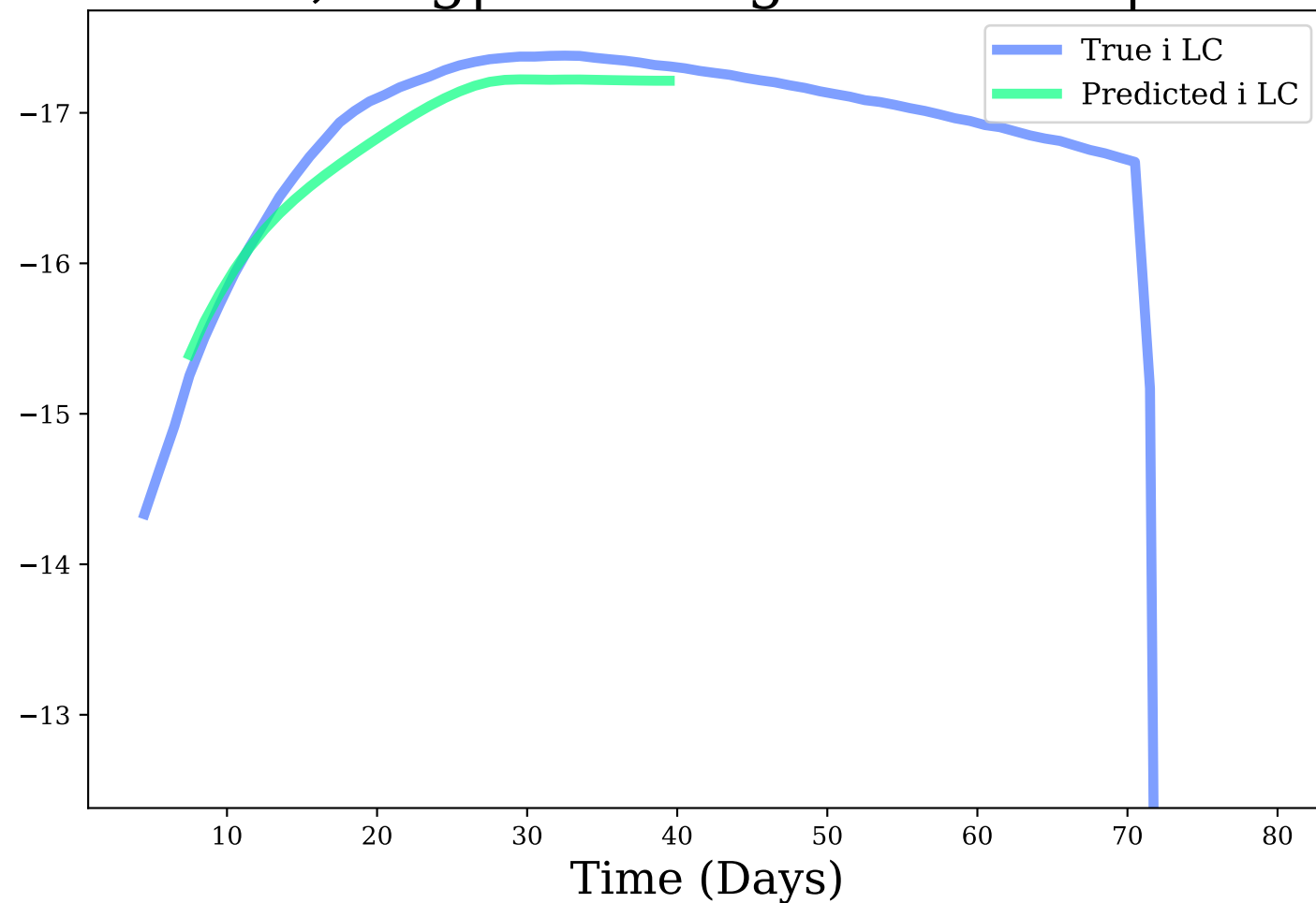
i-band, Avg|Max Mag Diff: 0.16 | 0.28
