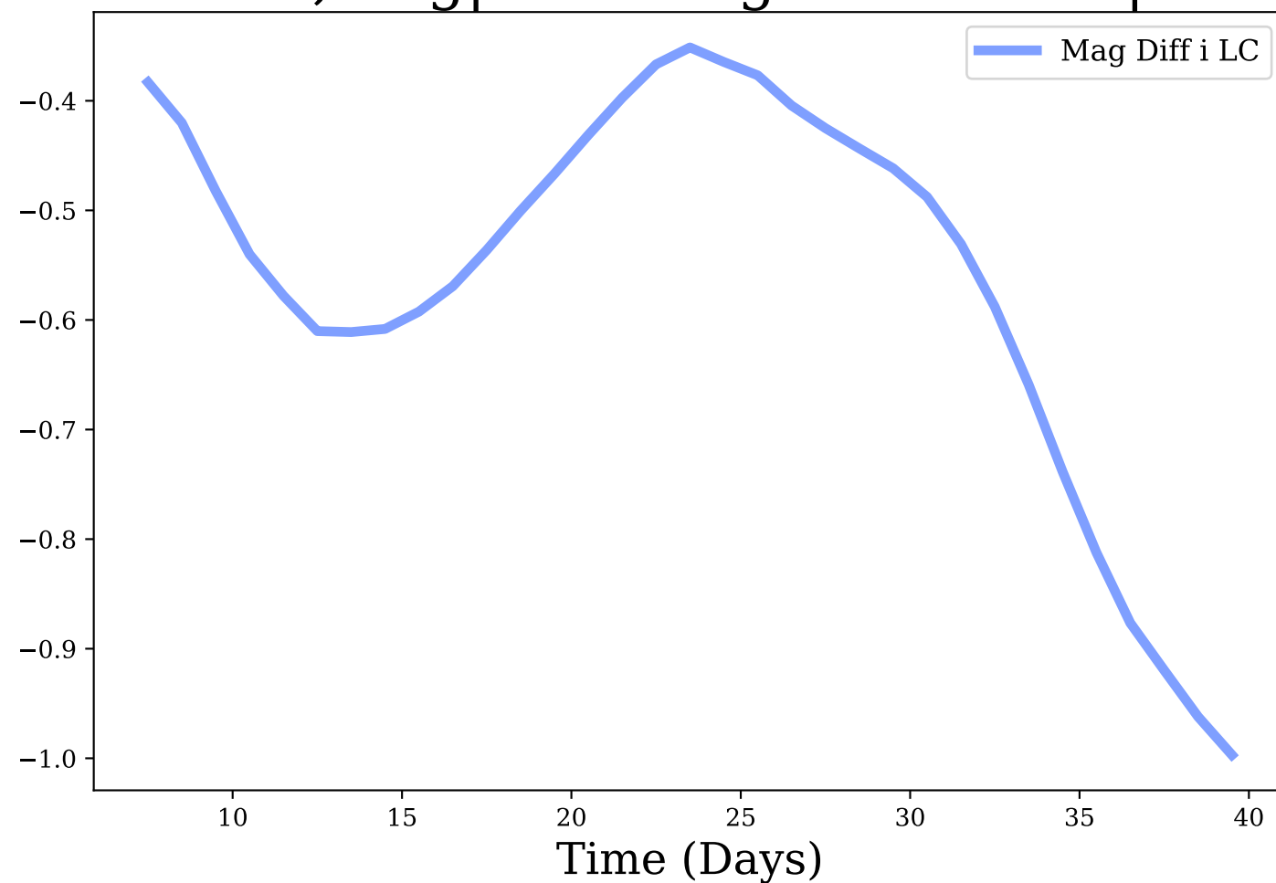
i-band, Avg|Max Mag Diff: -0.56 | 1.0
