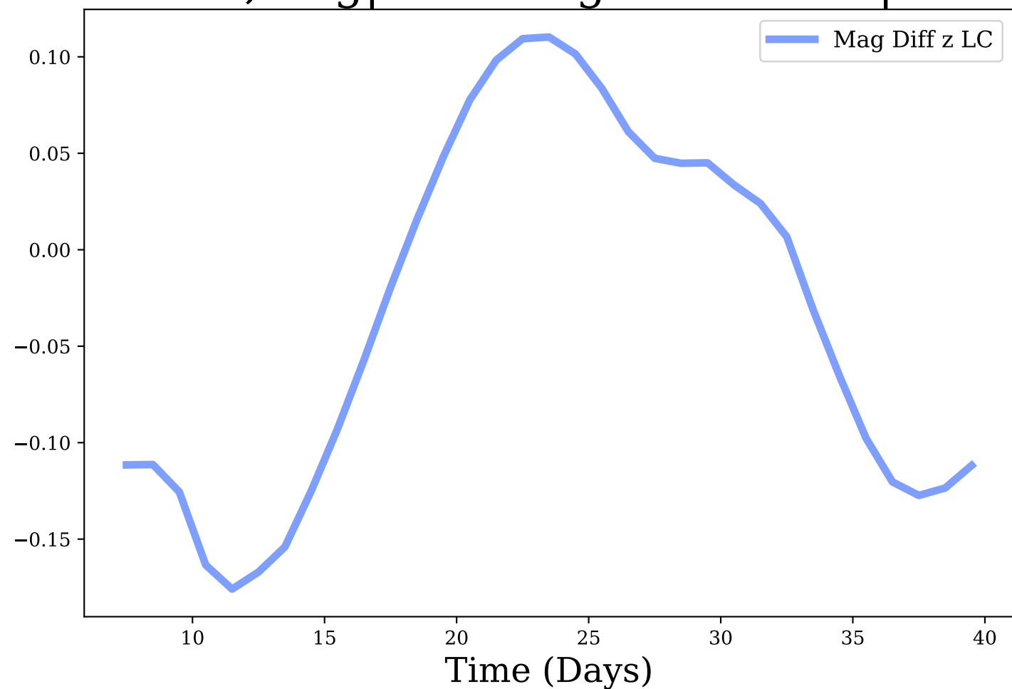
z-band, Avg|Max Mag Diff: -0.03 | 0.18
