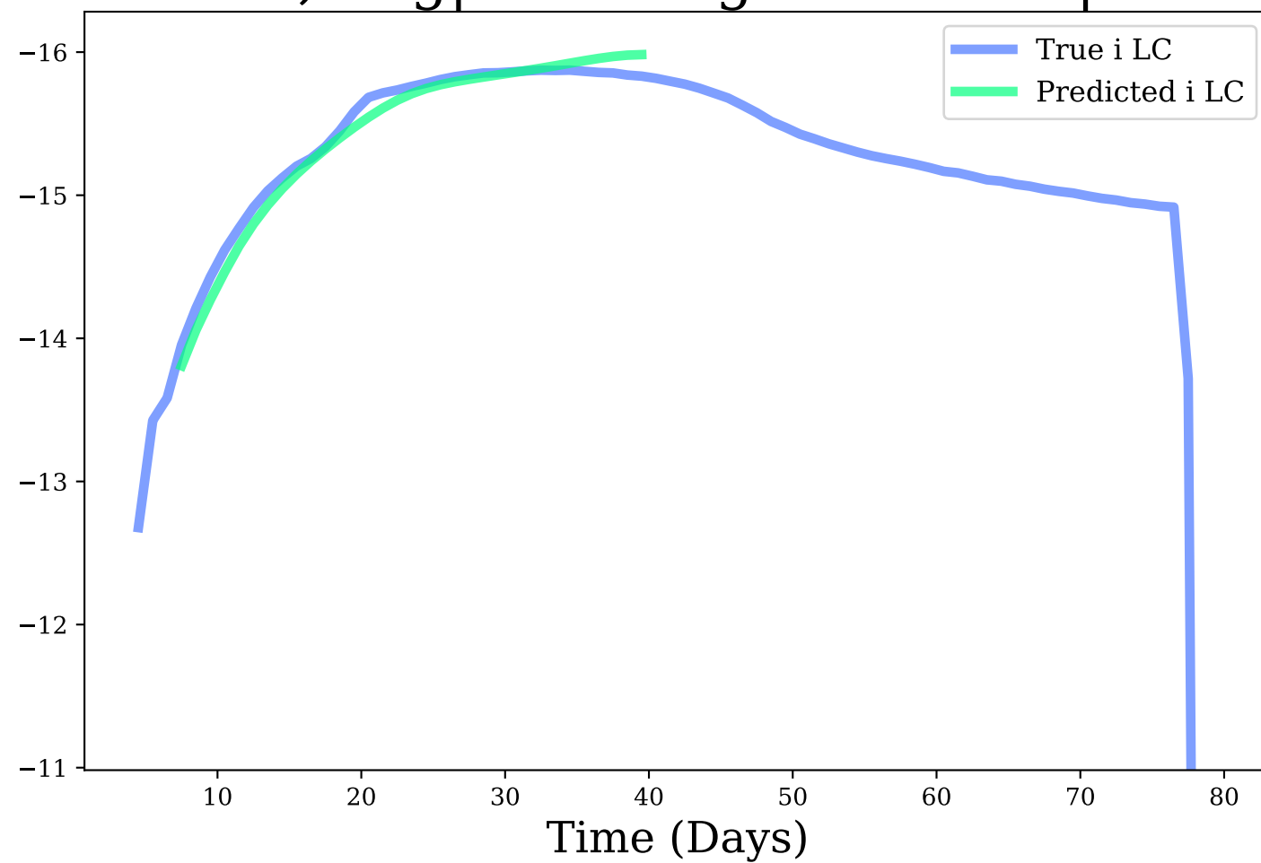
i-band, Avg|Max Mag Diff: 0.08 | 0.16
