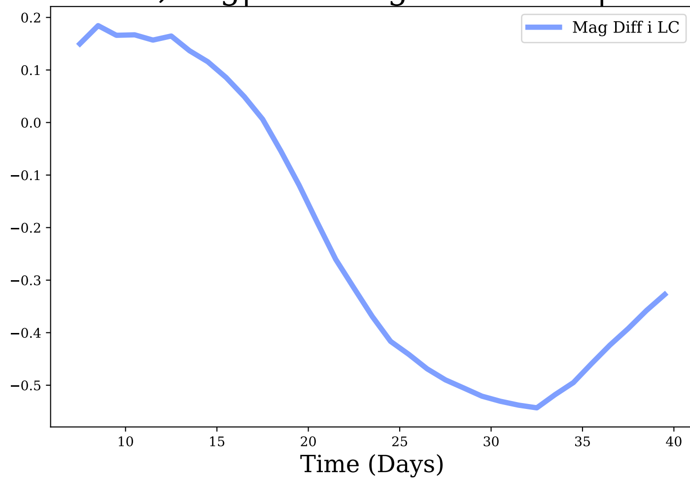
i-band, Avg|Max Mag Diff: -0.22 | 0.54
