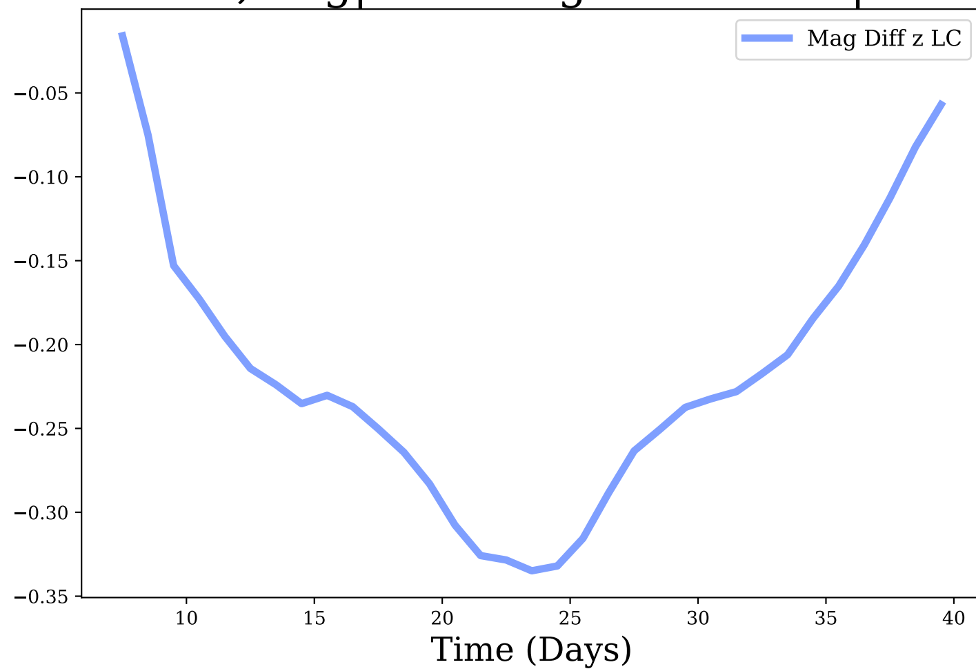
z-band, Avg|Max Mag Diff: -0.22 | 0.33
