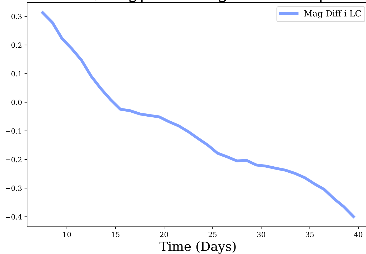
i-band, Avg|Max Mag Diff: -0.1 | 0.4
