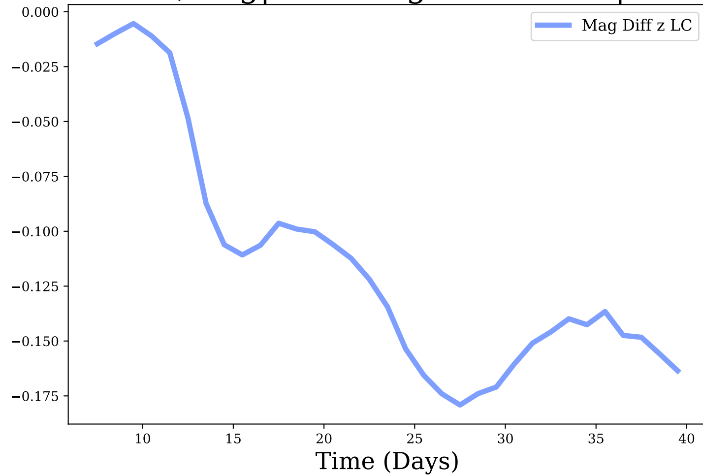
z-band, Avg|Max Mag Diff: -0.12 | 0.18
