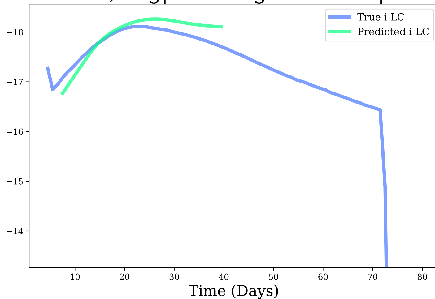
i-band, Avg|Max Mag Diff: 0.18 | 0.4
