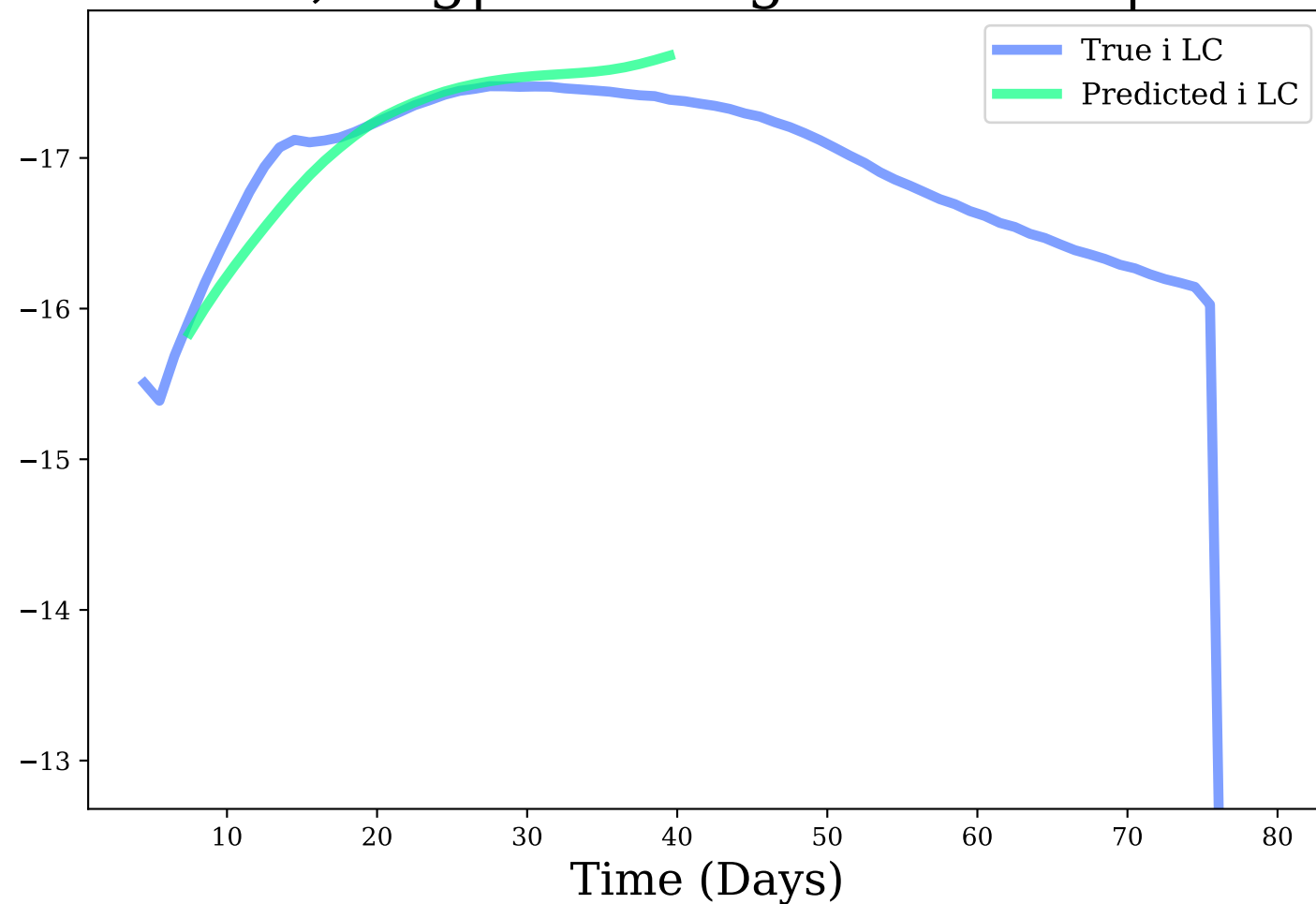
i-band, Avg|Max Mag Diff: 0.14 | 0.41
