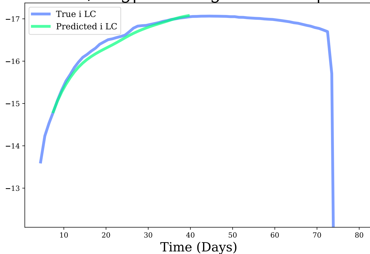
i-band, Avg|Max Mag Diff: 0.08 | 0.17
