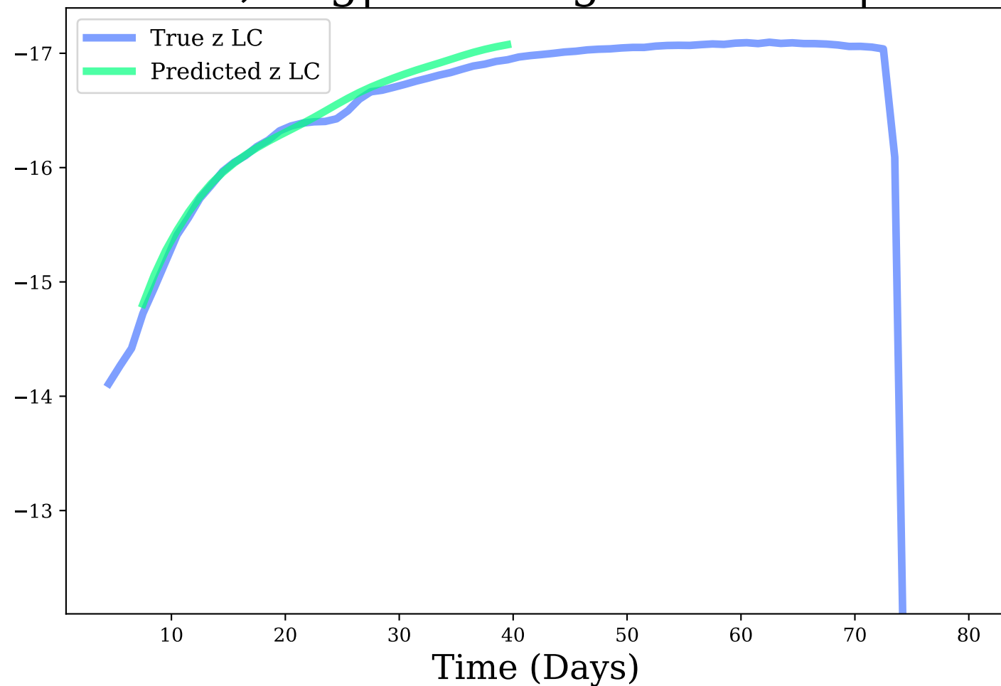
z-band, Avg|Max Mag Diff: 0.07 | 0.13
