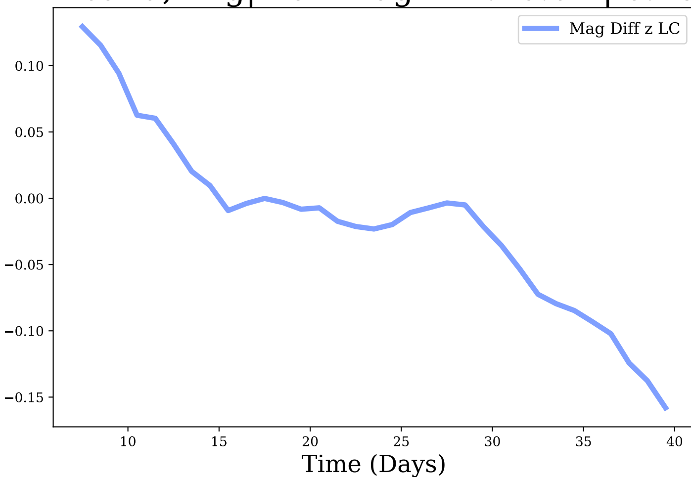
z-band, Avg|Max Mag Diff: -0.02 | 0.16
