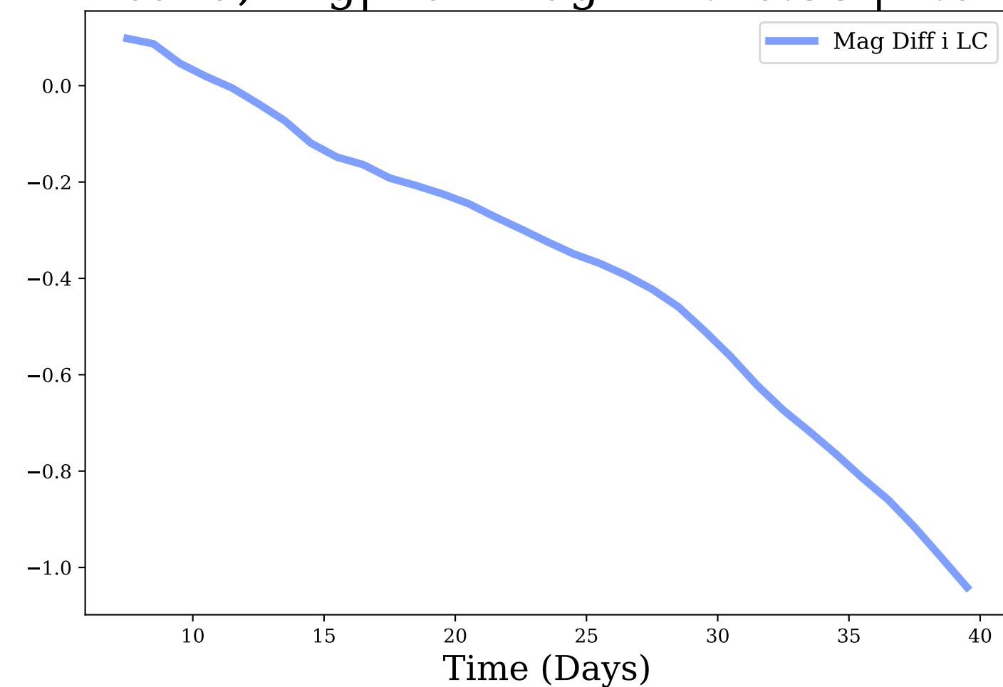
i-band, Avg|Max Mag Diff: -0.38 | 1.04
