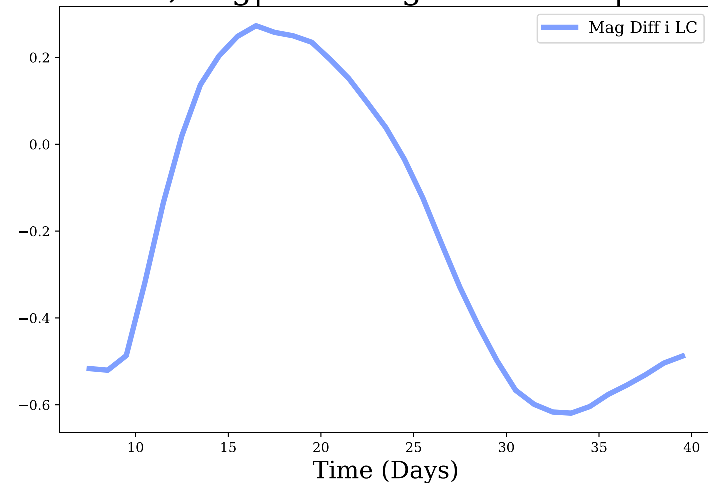
i-band, Avg|Max Mag Diff: -0.22 | 0.62
