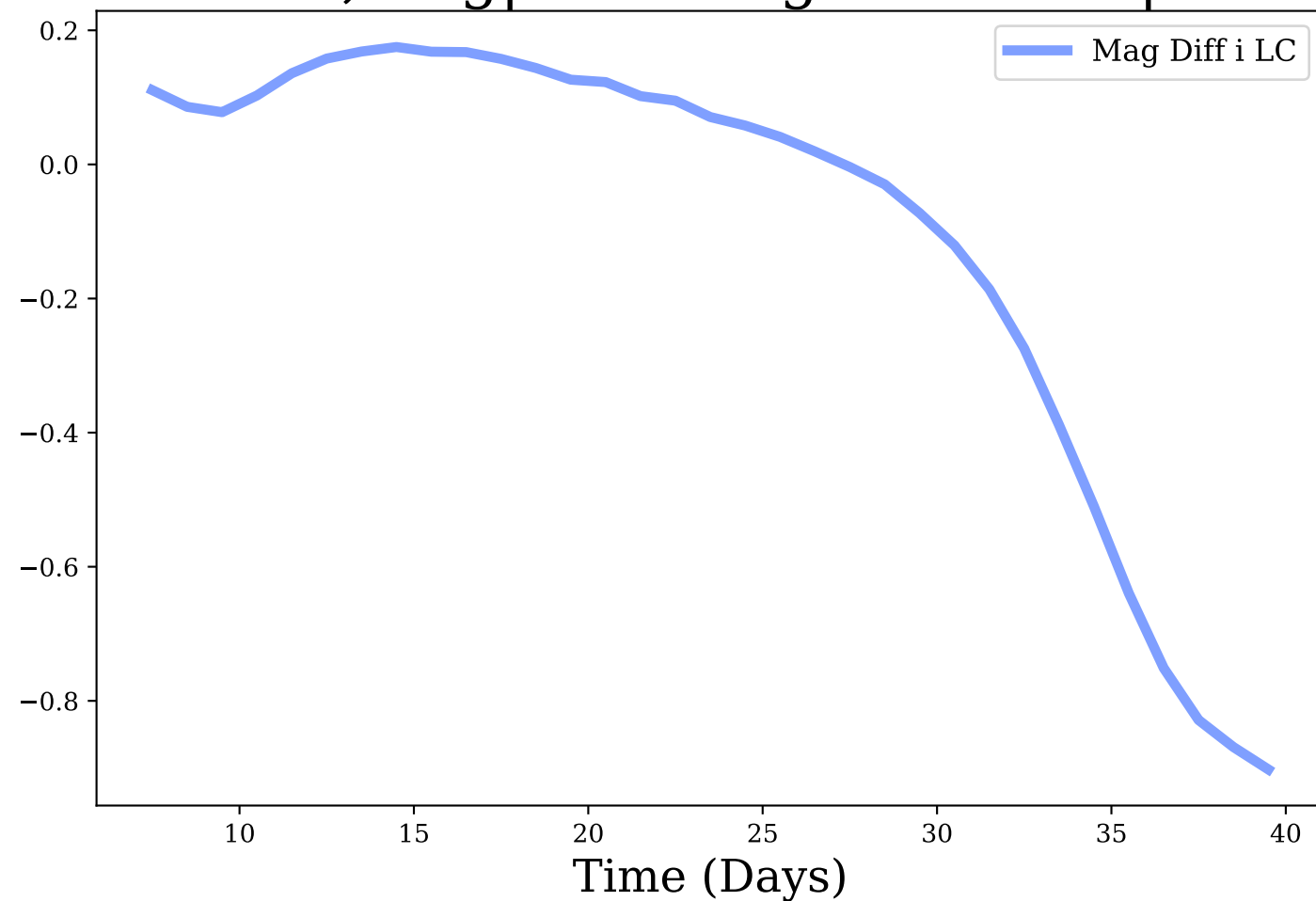
i-band, Avg|Max Mag Diff: -0.1 | 0.9
